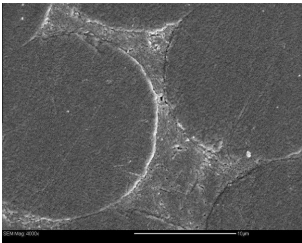
Fig. 18. Non-aged resin/PA yarn interface obtained by SEM (4000×).
