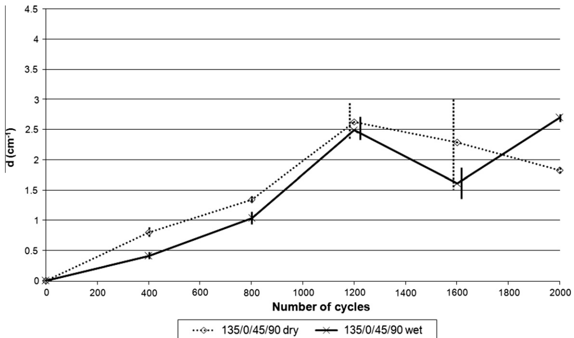
Fig. 12. Crack density versus the number of cycles for quasi-isotropic laminates.
