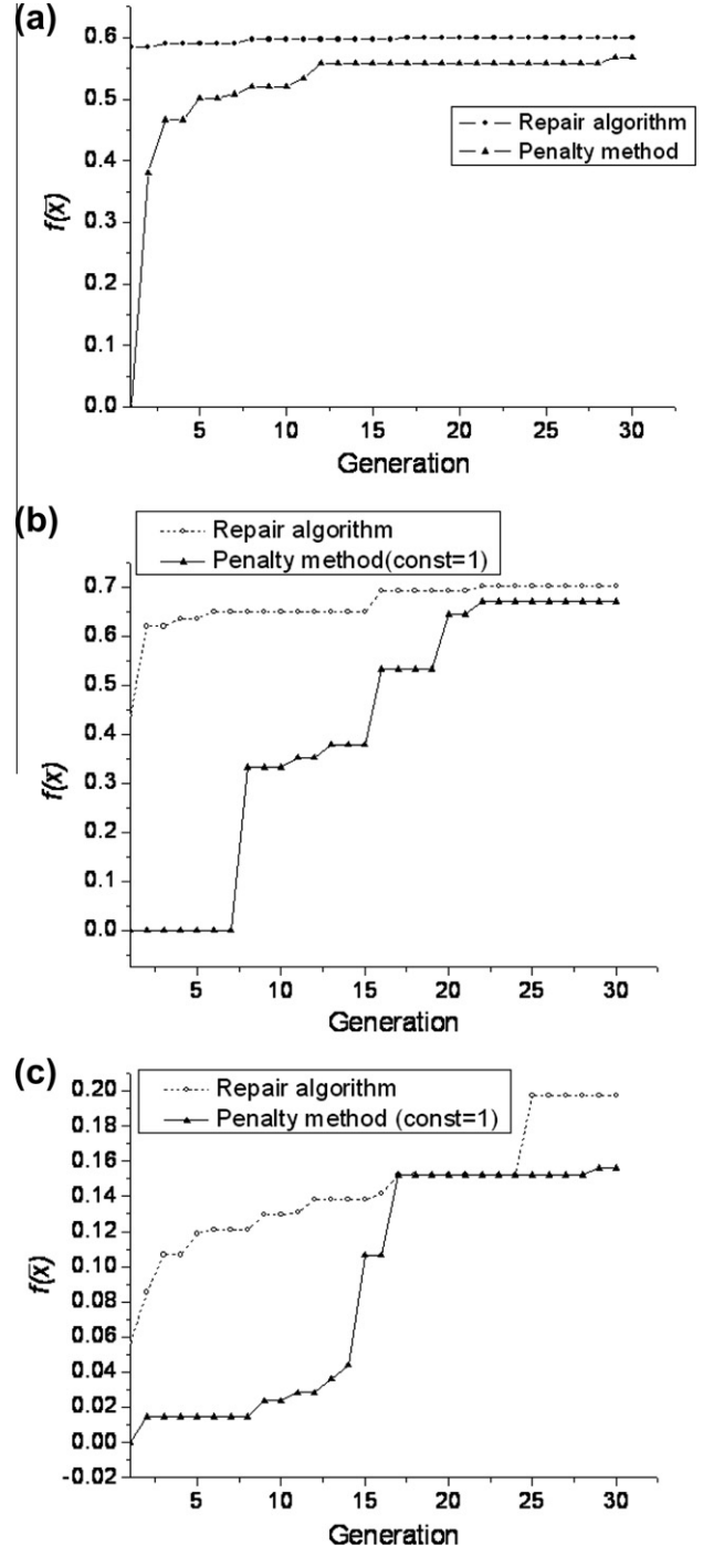
Fig. 9. Convergence test of repair algorithm and penalty method for (a) test function 1, (b) test function 2 and (c) test function 3.
