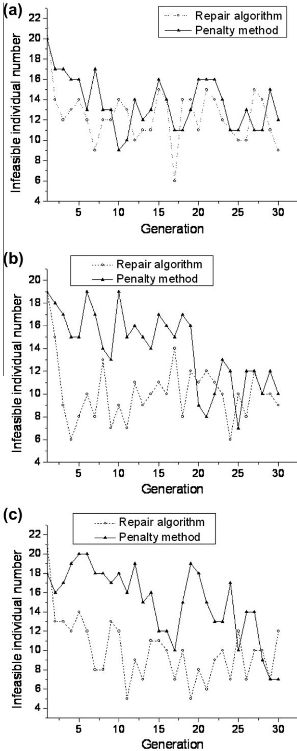
Fig. 10. Evolution of number of infeasible individuals for (a) test function 1, (b) test function 2 and (c) test function 3.
