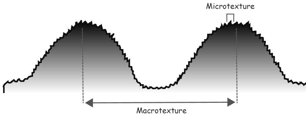
Figure 5 – The two scales of pavement texture
