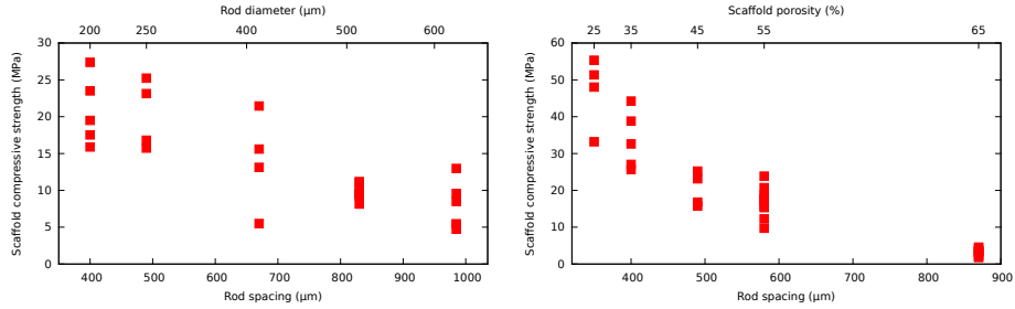
(a) Batch S_{V=45\%}^{\text{HA}} , i.e. HA scaffolds with constant porosity (45%) (b) Batch S_{d=250\mu\text{m}}^{\text{HA}} , i.e. HA scaffolds with constant rod diameter (250 \mu\text{m} before sintering)
