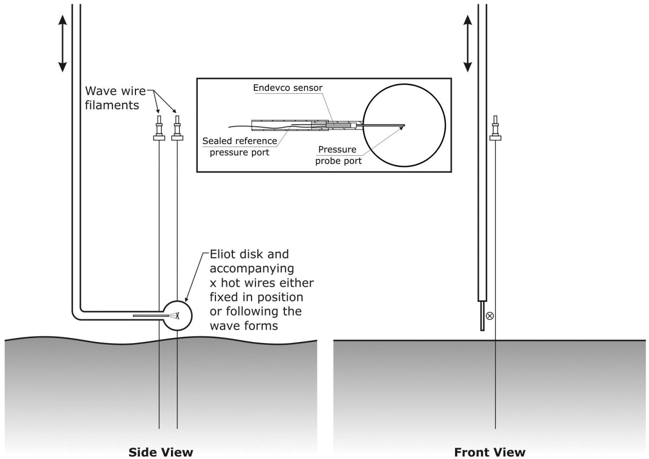
Figure 4. A sketch of the physical arrangement of the hot-wire/pressure probe mounted on the wave-follower in the large IRPHE facility. The X hot wire is mounted between the Elliot pressure disk and the two wave gauges. The inset figure is a sketch of the pressure probe. The pressure sensor is located 25\text{mm} downwind from the centre of the Elliot disk. Cross tank spacing between each instrument is 5\text{mm} .
