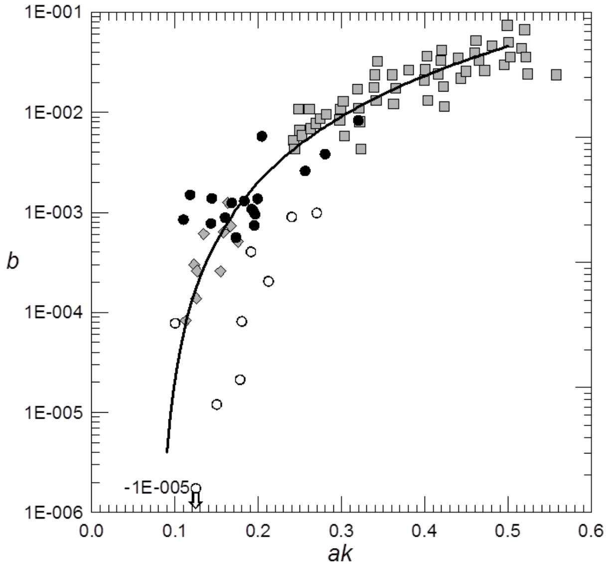
Figure 15. Breaking strength b expressed as a function of steepness ak . Data obtained from the present study is shown as solid circles, grey diamonds are data from Banner and Peirson (2007) and grey squares are data from Drazen et al. (2008). The equivalent non-breaking normalised dissipation rates are shown as hollow circles. The solid line is the fit b = 0.4(ak - 0.08)^{5/2} from Romero et al. (2012).
