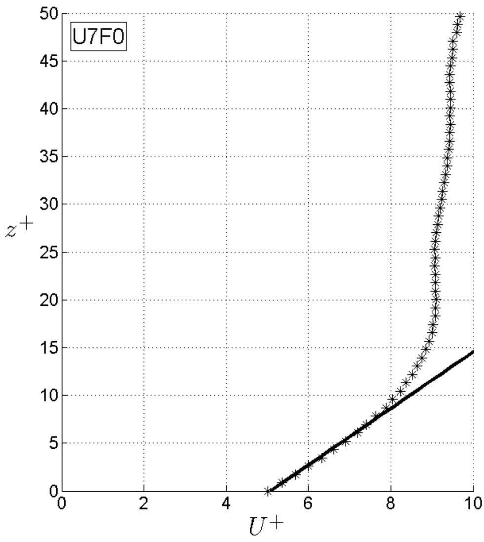
Figure 3. Representative wall-normalised velocity profile obtained in large IRPHE facility from the kingfisher and shows a near-instantaneous determination of the tangential stress.
