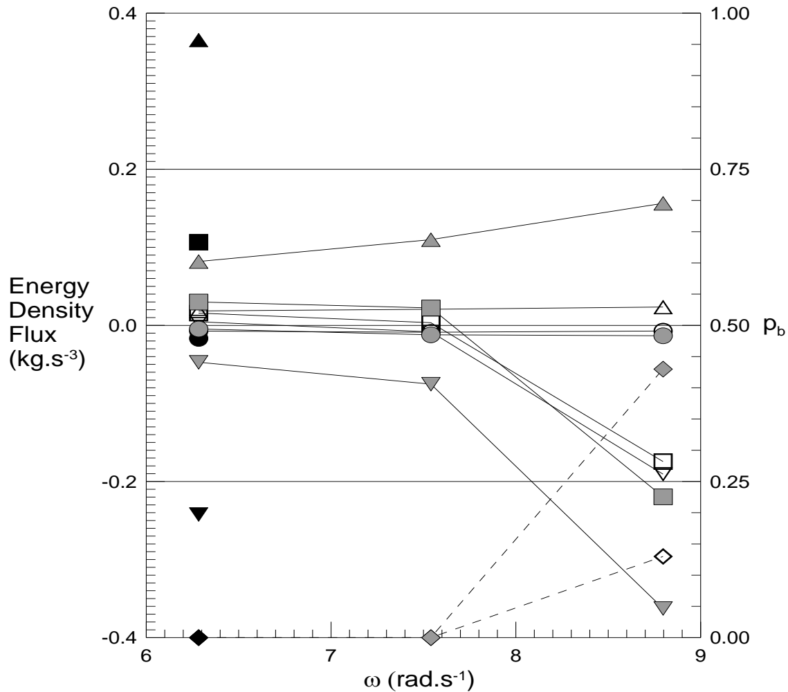
Figure 12c. Energy budget for monochromatic waves in the large IRPHE facility as a function of wind speed and wave frequency:
