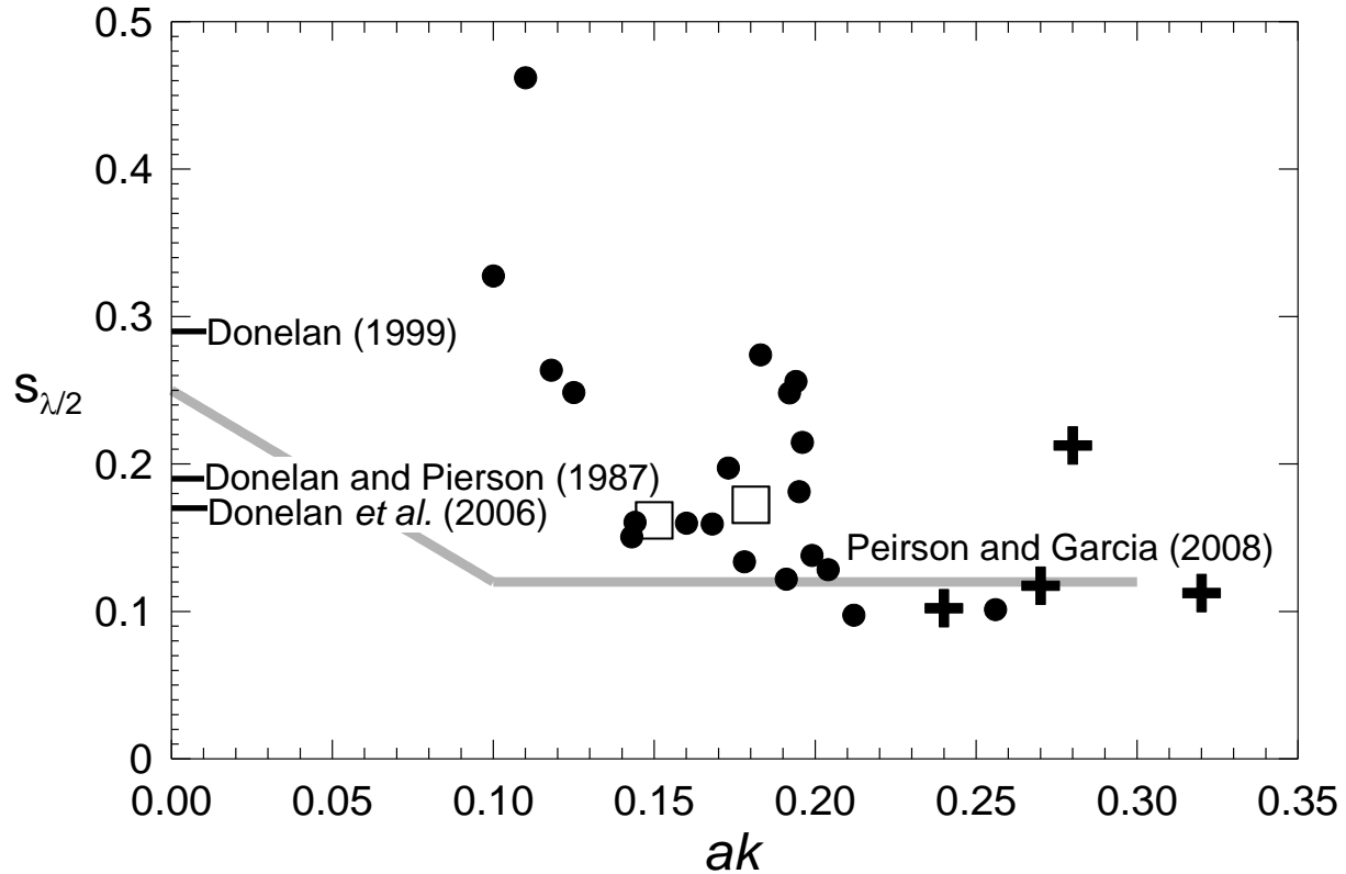
Figure 11. Normalised wind energy input rate, expressed as Jeffreys sheltering coefficients (Equation (9)), as a function of mean wave steepness. Hollow squares are data from Mastenbroek et al. (1996), solid circles are obtained from viscous measurements using the kingfisher in the large IRPHE facility (Grare 2009) and the crosses are values measured using PIV techniques in the small WRL facility (Peirson et al. 2012b). The grey line indicates the approximate mean values determined by Peirson and Garcia (2008) based on measurements of net wave growth. Solid lines at ordinate axis indicate sheltering coefficients determined by Donelan and Pierson (1987), Donelan (1999) and Donelan et al. (2006).
