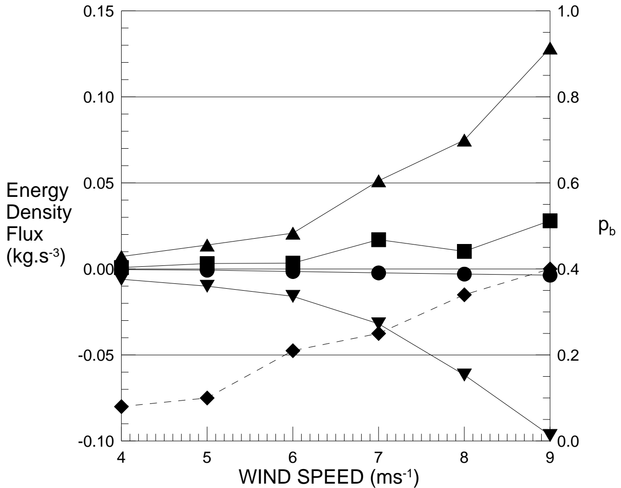
Figure 12b. Energy budget for wind waves in the large IRPHE facility at 28m fetch as a function of wind speed:
