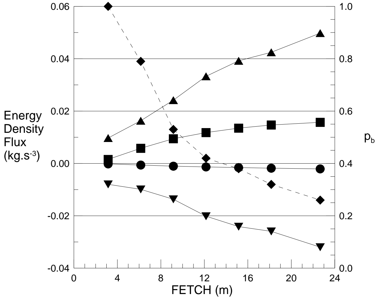
Figure 12a. Energy budget for wind waves in the large IRPHE facility at 7ms^{-1} wind speed as a function of fetch.
