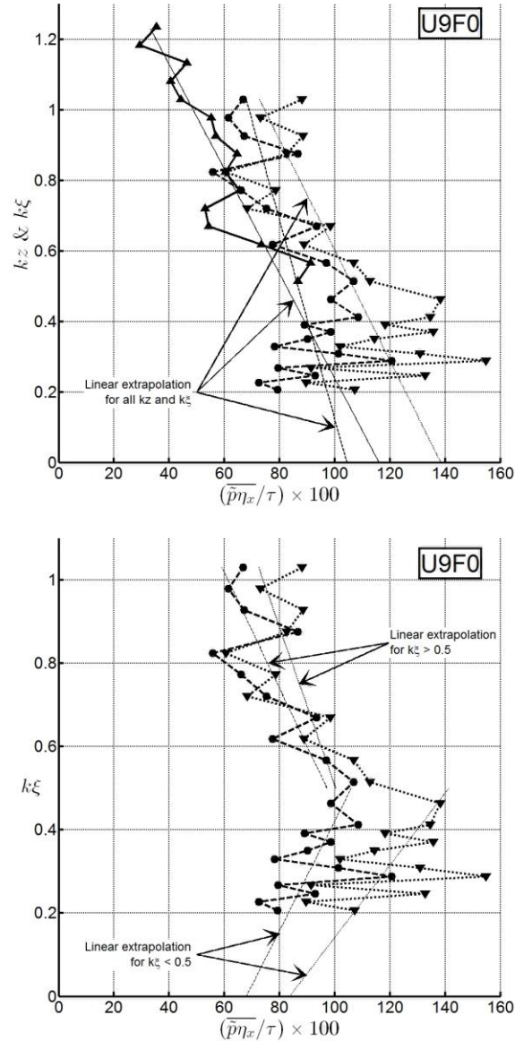
Figure 6. Vertical profiles of normalized pressure/wave slope correlation, and extrapolations of the normalized form drag at the water surface for the case U9F0.
