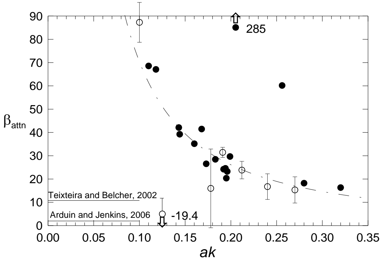
Figure 13. Normalised energy loss as a function of wave steepness. Hollow circles are non-breaking waves and solid circles are breaking wave cases. Corresponding estimates by Teixeira and Belcher (2002) and Arduin and Jenkins (2006) are shown as solid lines on the ordinate axis. The dash-dotted line indicates the best power fit of the data \beta_{attn} = 2.62(ak)^{-1.43 \pm 0.21} .
