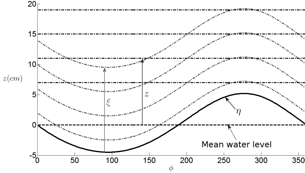
FIGURE A.1 – Cartesian and curvilinear wave following frames
