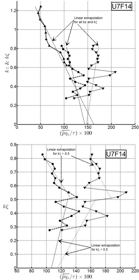
Figure 7. Vertical profiles of normalized pressure/wave slope correlation, and extrapolations of the normalized form drag at the water surface for the case U7F14.
