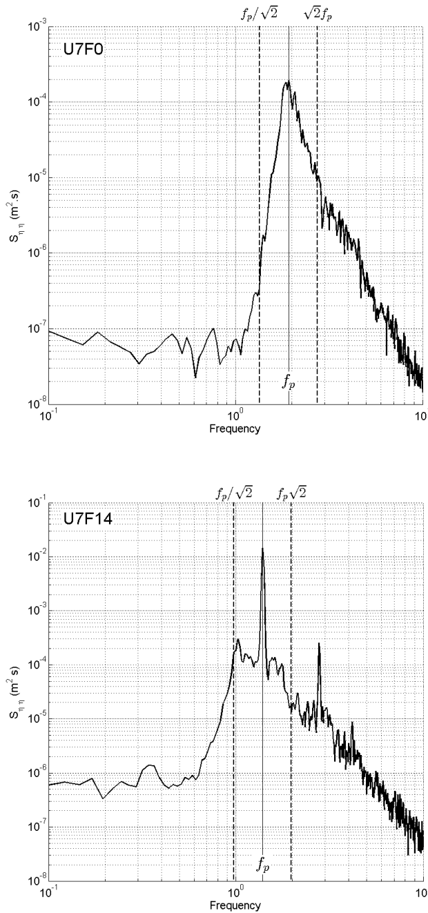
Figure 1. Spectra of the water surface elevation signal. Upper panel: pure wind wave case ( U_m = 7 \text{ m} \cdot \text{s}^{-1} ). Lower panel: mechanically generated case ( f_m = 1.4 \text{ Hz} , and U_m = 7 \text{ m} \cdot \text{s}^{-1} ). The vertical dotted lines represent the boundaries of the frequency range \omega_p/\sqrt{2} < \omega < \sqrt{2}\omega_p where \omega_p = 2\pi f_p is the spectral peak frequency of the dominant waves. This frequency range was found to encapsulate over 92% of the total spectral energy of the surface elevation for all the cases studied.
