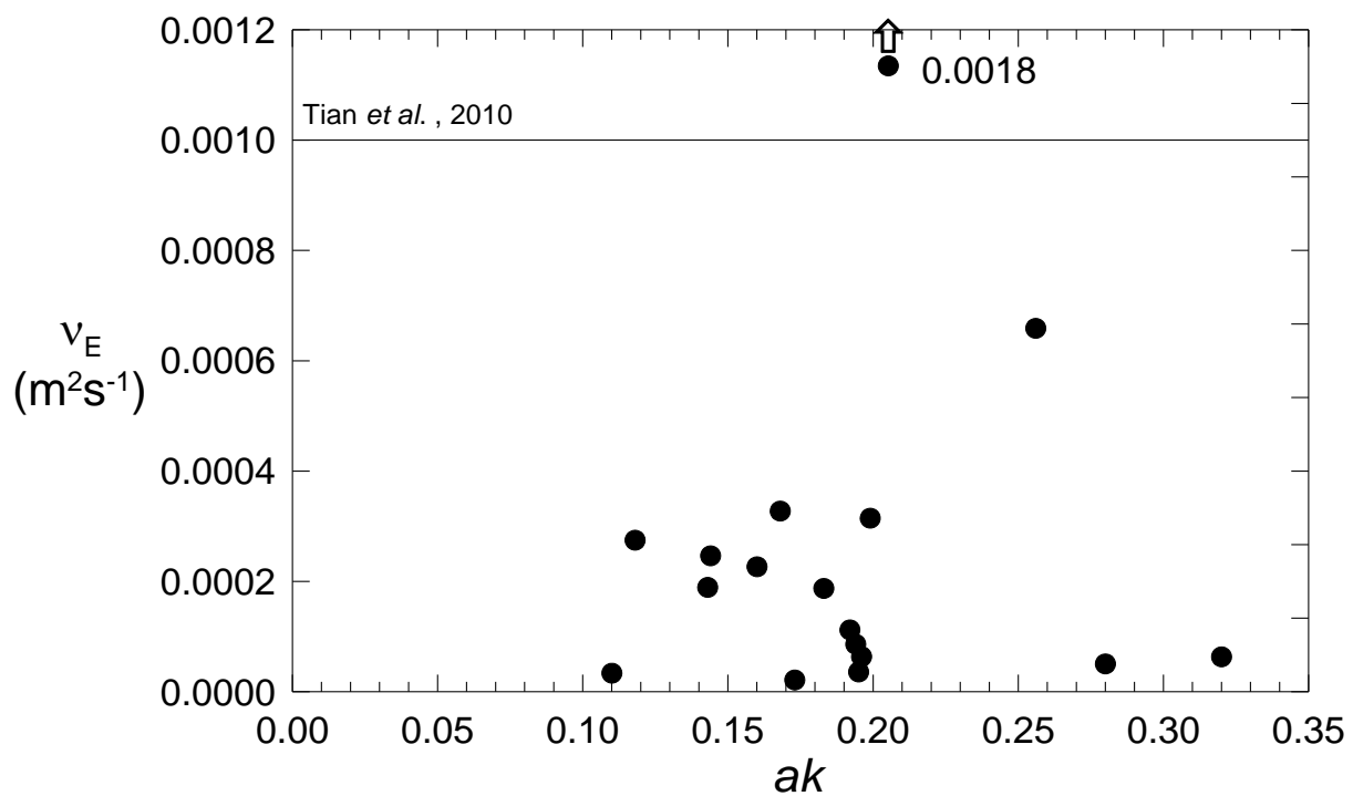
Figure 14. Eddy viscosity during active breaking as defined in equation (41).
