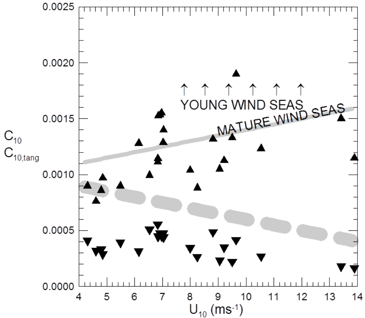
Figure 8. Comparison of tangential stresses with Banner and Peirson (1998).
