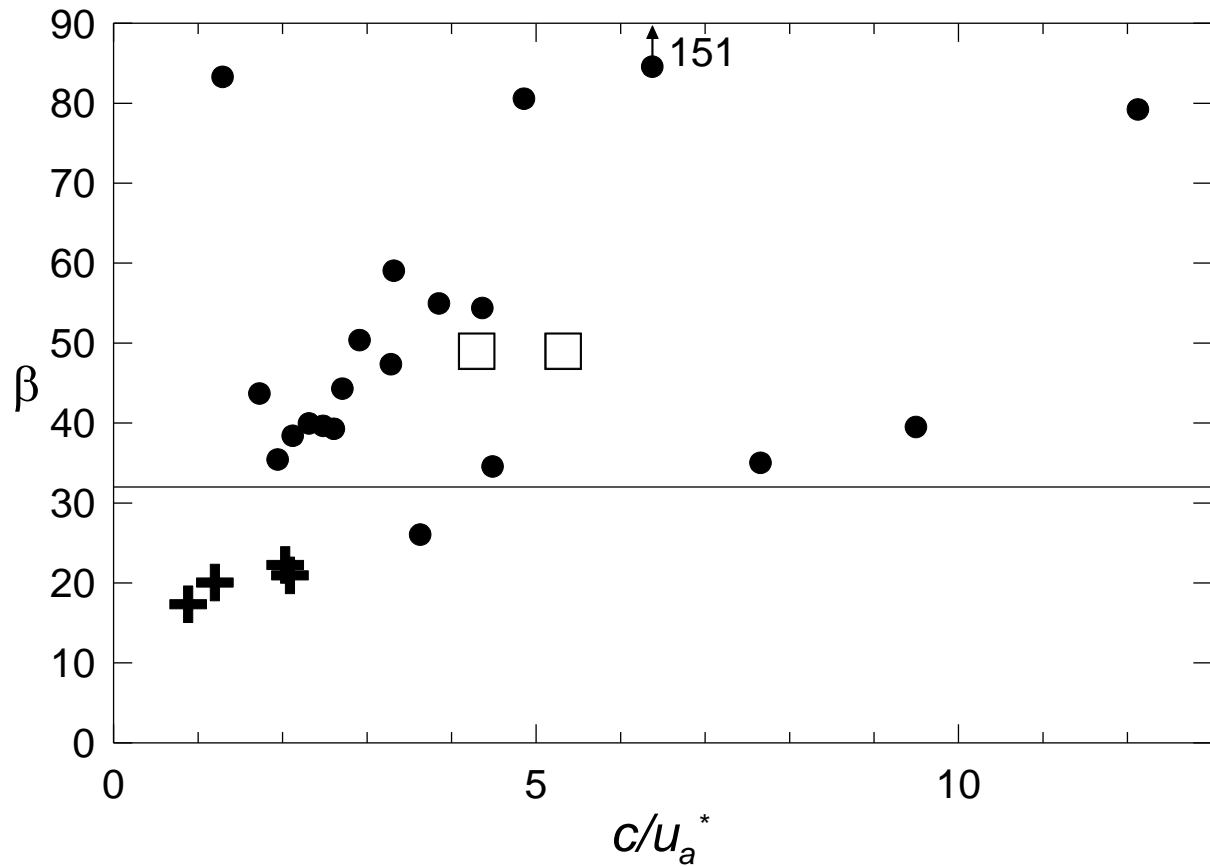
Figure 10. Normalised wind energy input rate expressed as function of wave age. Hollow squares are data from Mastenbroek et al. (1996), solid circles are obtained from viscous measurements using the kingfisher in the large IRPHE facility (Grare 2009) and the crosses are values measured using PIV techniques in the small WRL facility (Peirson et al. 2012b). The solid line indicates the conventional mean value of Plant (1982).
