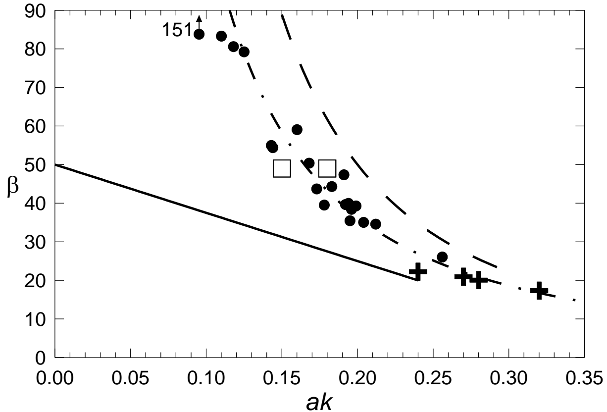
Figure 9. Normalised wind energy input rate expressed as function of mean wave steepness. Hollow squares are data from Mastenbroek et al. (1996), solid circles are obtained from viscous measurements using the kingfisher in the large IRPHE facility (Grare 2009) and the crosses are values measured using PIV techniques in the small WRL facility (Peirson et al. 2012b). The dashed line indicated the theoretical limit \beta = 2/(ak)^2 and the solid line indicates the mean values of net wave growth determined by Peirson and Garcia (2008). The dash-dotted line indicates the best power fit of the data: \beta = 2.56(ak)^{-1.65 \pm 0.11} .
