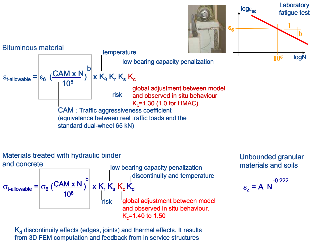
Figure 4: General expression of the allowable strain and strain values
