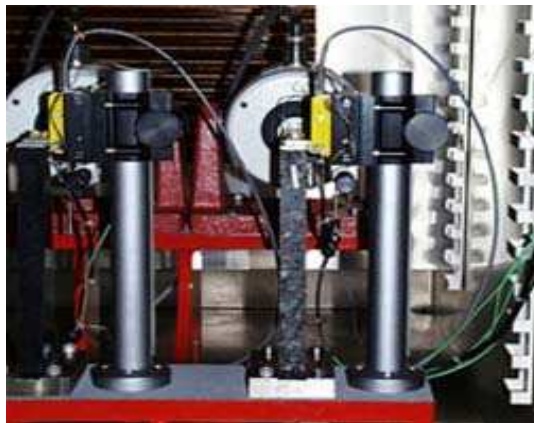
Figure 3: fatigue test on bituminous material (Trapezoidal 2 point beam flexion)
