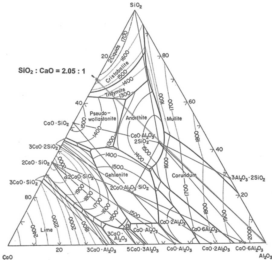
Fig. 12. Phase diagram of the ternary system Al 2 O 3 –CaO–SiO 2 . 24
