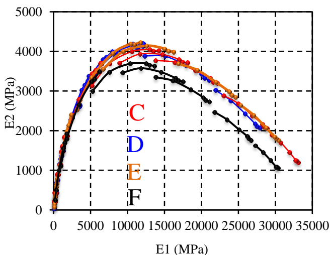
Figure 5: Cole-Cole results for mixes C to F
