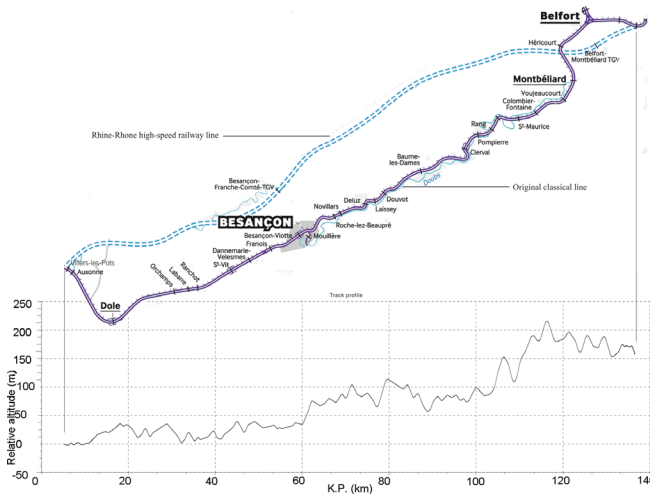
Figure 4 Map and track profile of the test section
