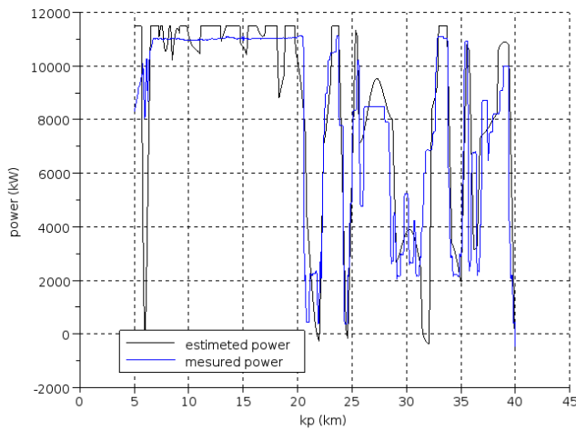
Figure 5 Modeled power versus measurements on a part of the test section
