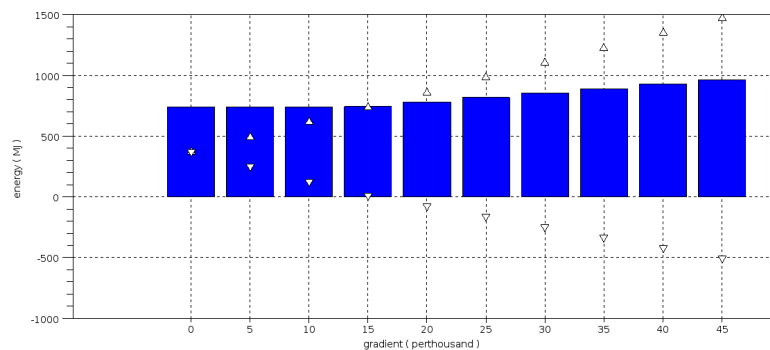
Figure 6 Modeling of the influence of longitudinal slopes (positives (Δ) and negatives (∇) slopes of increasing levels from 0 to 4,5 ‰)
