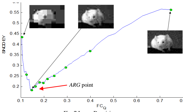
Fig. 7 Image Denoising
