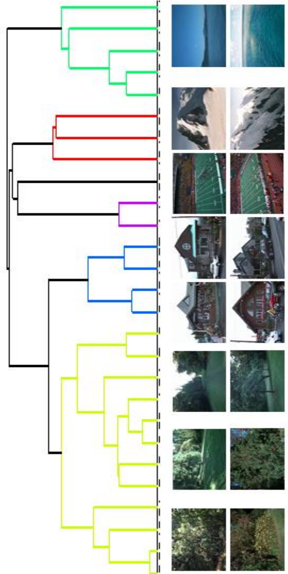
Fig. 1. Image Classification
