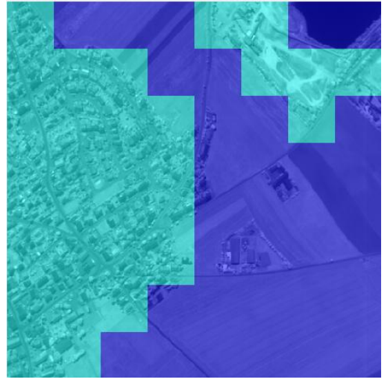
Fig. 2. Image Segmentation
