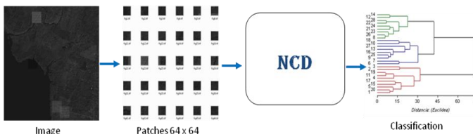
Fig. 11 Experiment Process: we take the satellite image and divide it into patches of 64 \times 64 pixels, with these patches we calculate the distance matrix between them using NCD and finally we applied a hierarchical classification method to cluster and identify the patches with artifacts
