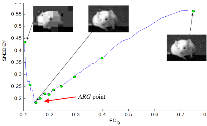
Fig. 7 Image Denoising
