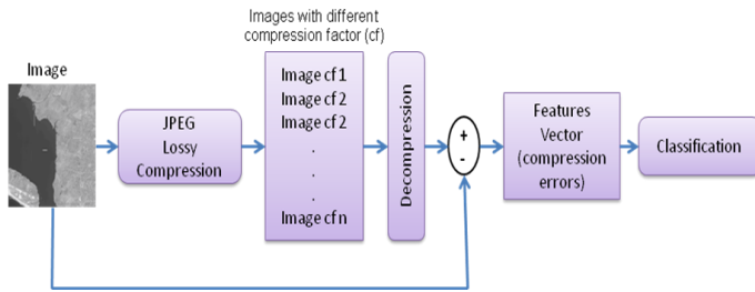
Fig. 8 Block Diagram for Rate-Distortion Analysis [10]
