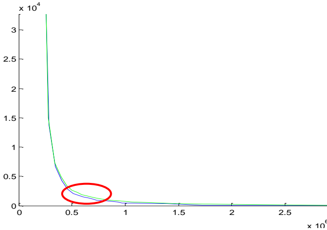
Fig. 5 Experimental KSF curve, the horizontal axis represents the Kolmogorov complexity approximation as the size of the image compressed file in bytes, the vertical axis represents the amount of bits that is needed to represent a model of original image. Blue for Figure 3 (a) and green for Figure 3 (b), the KSF experimental curve of the original image is different from the experimental curve KSF for image that contains manipulations. [6]
