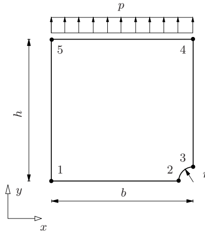
Figure 14: Square plate with a circular hole taking advantage of symmetry
