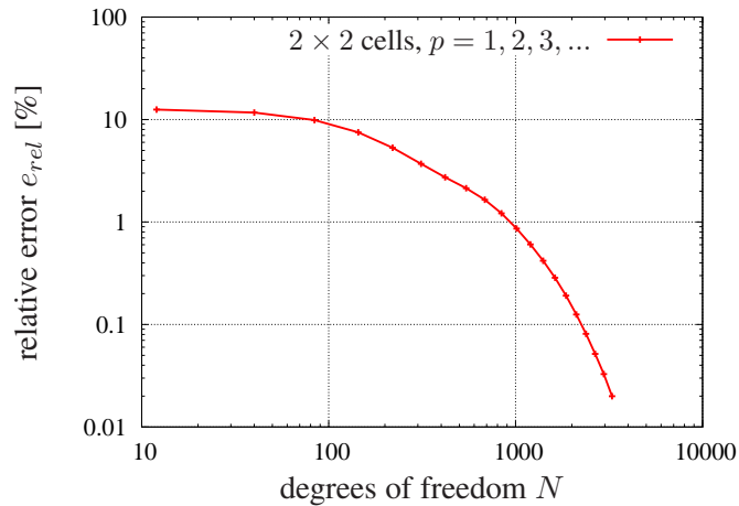
Figure 16: Convergence of the error in energy norm for a p -extension on 2 \times 2 cells
