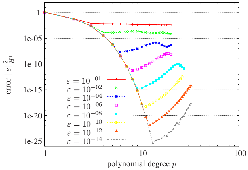
Figure 10: p -Extension on mesh with three elements for different \varepsilon values
