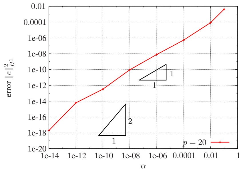
Figure 11: Influence of \alpha on the error
