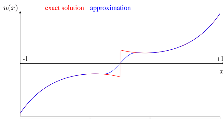
Figure 6: Comparison of exact solution and FCM approximation with p = 20 and \alpha = 10^{-14}
