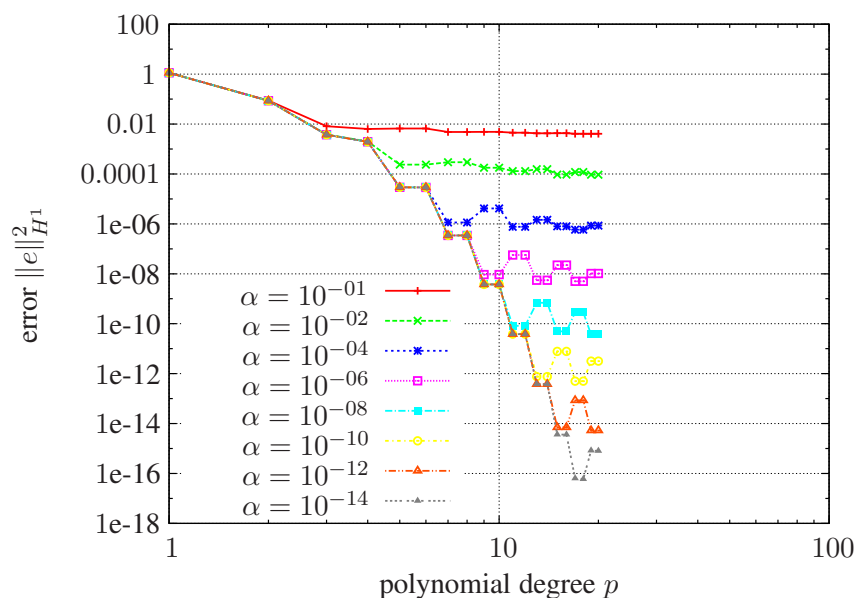
Figure 7: p -Extension on mesh with three elements for different \alpha values
