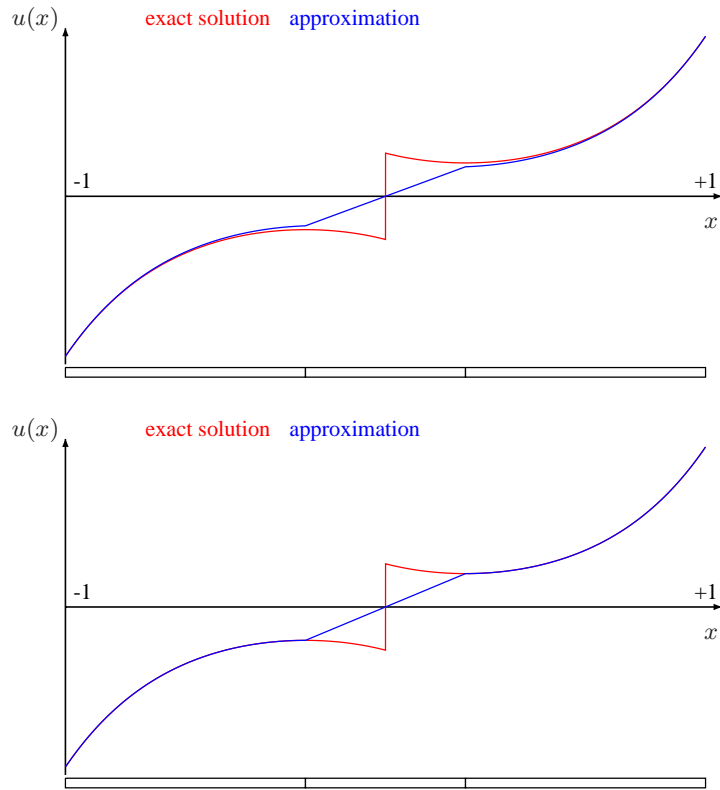
Figure 3: Comparison of exact solution and FCM approximation with p = 20 and \alpha = 10^{-01} (upper part) and \alpha = 10^{-14} (lower part)
