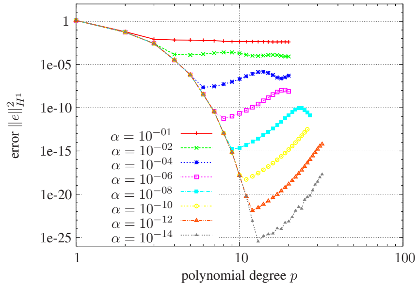
Figure 10: p -Extension on mesh with three elements for different \alpha values
