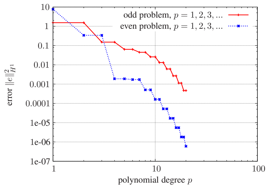
Figure 2: p -Extension on mesh with one element, \alpha = 0 , exact integration
