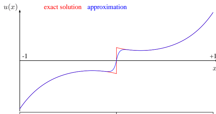
Figure 12: Comparison of exact solution and FCM approximation with p = 20 and \alpha = 10^{-14}
