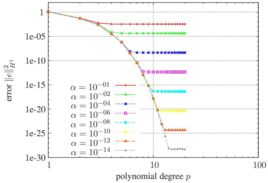
Figure 4: p -Extension on a mesh with three cells for different values of \alpha
