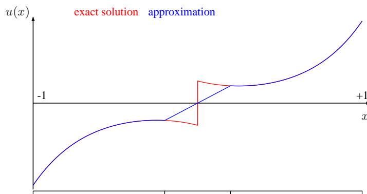
Figure 9: Comparison of exact solution and FCM approximation with p = 20 and \alpha = 10^{-14}
