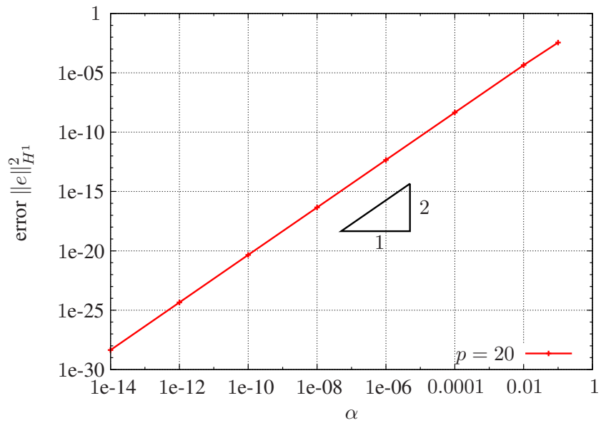
Figure 5: Influence of \alpha on the error
