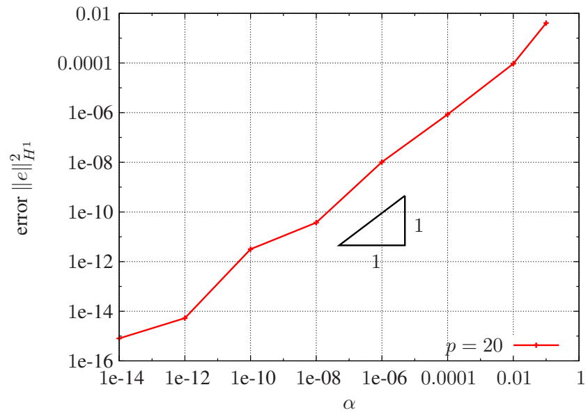
Figure 8: Influence of \alpha on the error
