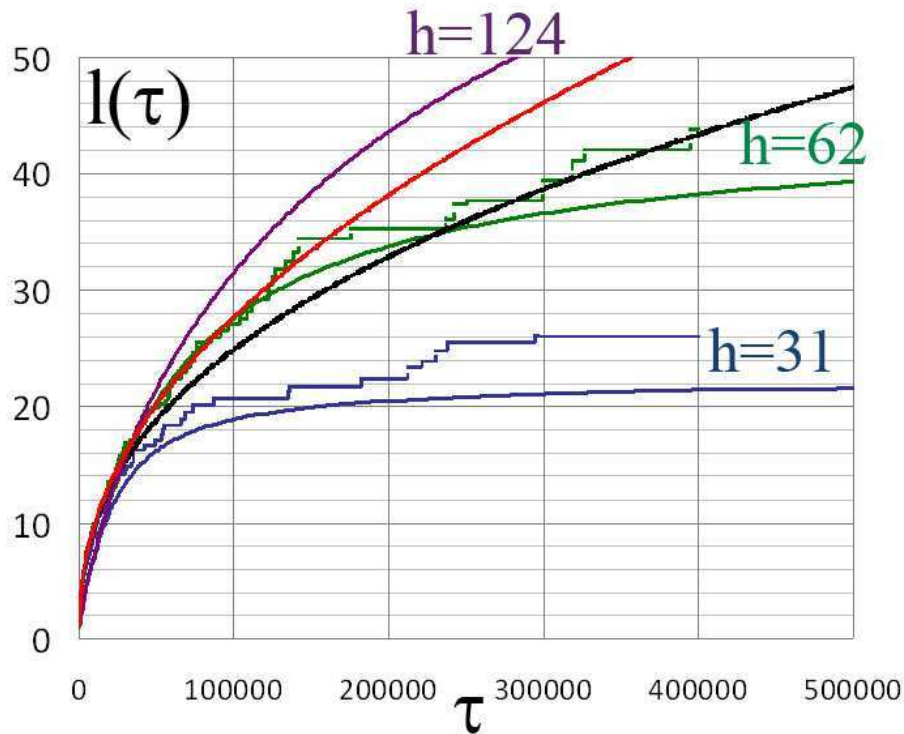
Fig.2 Average dimensionless length of the chains vs. the dimensionless time for the particle surface fraction \phi=8.91\% . Blue and green lines stand respectively for a box of 31 particle diameter and 62 diameters. The staircase shape is the numerical simulation result and the solid line is the solution of Eq.1. The purple solid line is the solution of Eq.(1) for a box of height 124 diameters. The black solid line is the 2D version of the model [2]. At last, the tiny red curve is the fit of the simulation with h=62 by a power law for l(\tau) < 20
