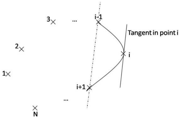
Figure 8. Definition of bicubic splines upon the initial point set for further interpolation
