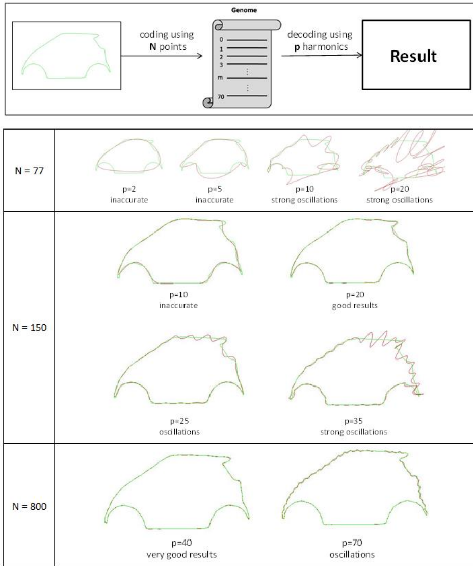
Figure 9. Comparison of silhouettes after interpolation with N points, encoding with p harmonics and decoding
