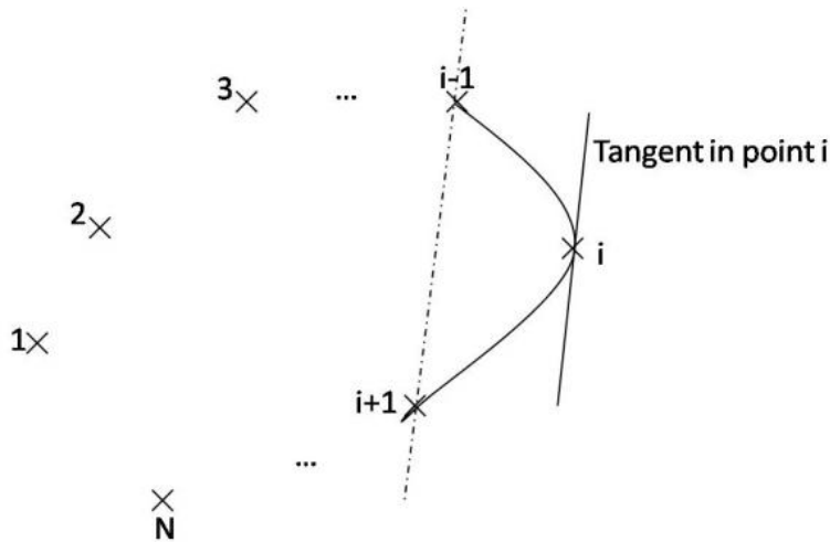
Figure 8. Definition of bicubic splines upon the initial point set for further interpolation
