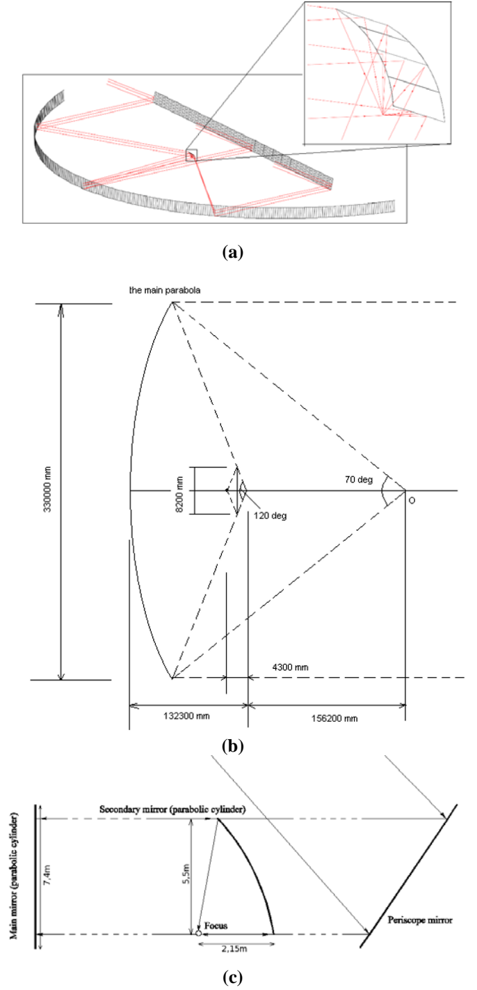
Fig. 1. The primary and secondary reflectors of the RATAN-600 radiotelescope (south sector): (a) Schematic 3D view; (b) Horizontal cut; (c) Vertical cut.
