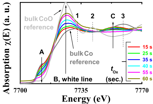
FIG. 5. Co-K edge XANES normalized profiles for as-deposited Pt/Co/AlO x trilayers and oxidized for different oxidation time t_{\text{ox}} . Note the evolutions of typical peaks [A (pre-edge), B (white line), and C] as a function of t_{\text{ox}} . Bulk references for Co and CoO are added for comparison. The 60 s is slightly shifted towards positive absorption for clarity of presentation (very close to the 55 s line).
