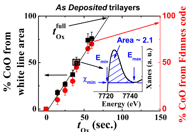
FIG. 6. Normalized white line area (left), corresponding to the normalized peak B appearing in Fig. 5, and content of CoO deduced from ab initio simulations 40 (right) versus t_{\text{ox}} for as-deposited Pt/Co/AlO x trilayers. Inset: Example of integration of the white line (normalized intensity) for t_{\text{ox}} = 40 s with the values for the energy ( E_{\text{min}} and E_{\text{max}} ) and the minimal XANES normalized intensity ( \chi_{\text{min}} ) used for calculating the areas.
