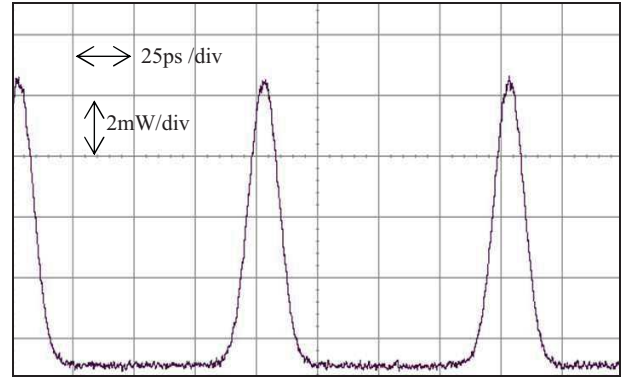
Fig. 2. Oscilloscope trace of the output pulse train.
