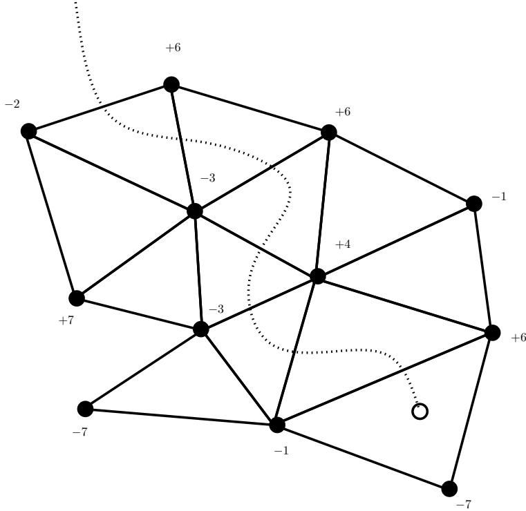
FIGURE 2. Fan's lemma in dimension 2: A part of a path followed by the algorithm finding another boundary alternating simplex or an alternating 2-simplex
