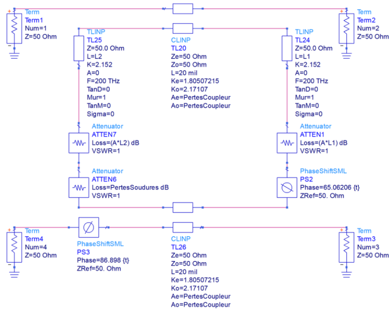
Fig. 5. FRR model created using ADS.
