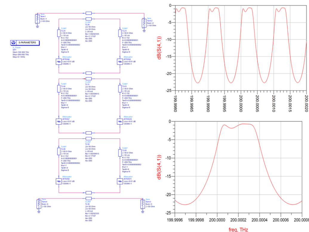
Fig. 7. ADS model and transmission response simulation results of a high rejection optical filter based on three compound FRRs with a total length of less than 1 meter.
