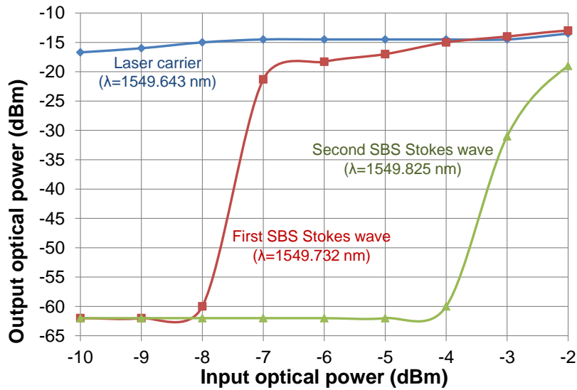
Fig. 10. Optical power measurements of the laser carrier and of both first and second stimulated Brillouin scattering Stokes waves, at the second and third outputs of the 20m-long FRR, versus the laser input power.
