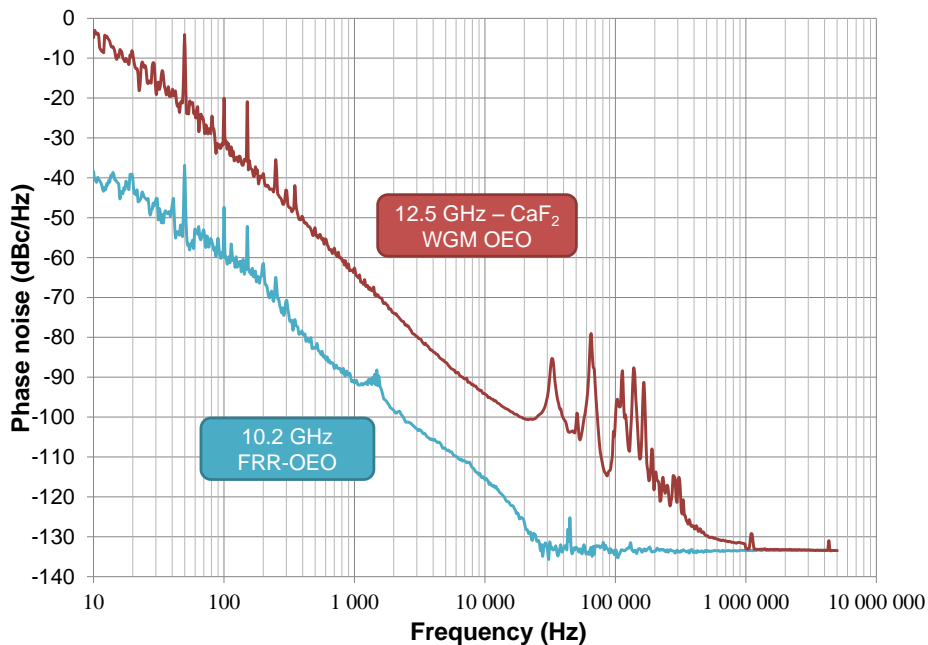
Fig. 11. Phase noise of OEOs based on a 20m-long fiber ring resonator (10.2 GHz) and a \text{CaF}_2 micro-resonator (12.5 GHz). Measurements were performed using an Agilent E5052 B signal source analyzer.
