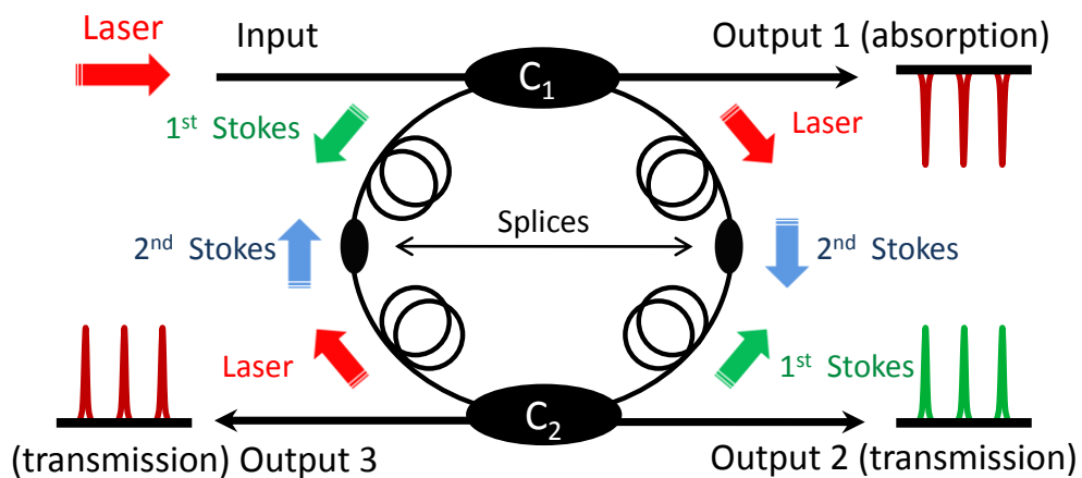
Fig. 4. Fiber ring resonator.
