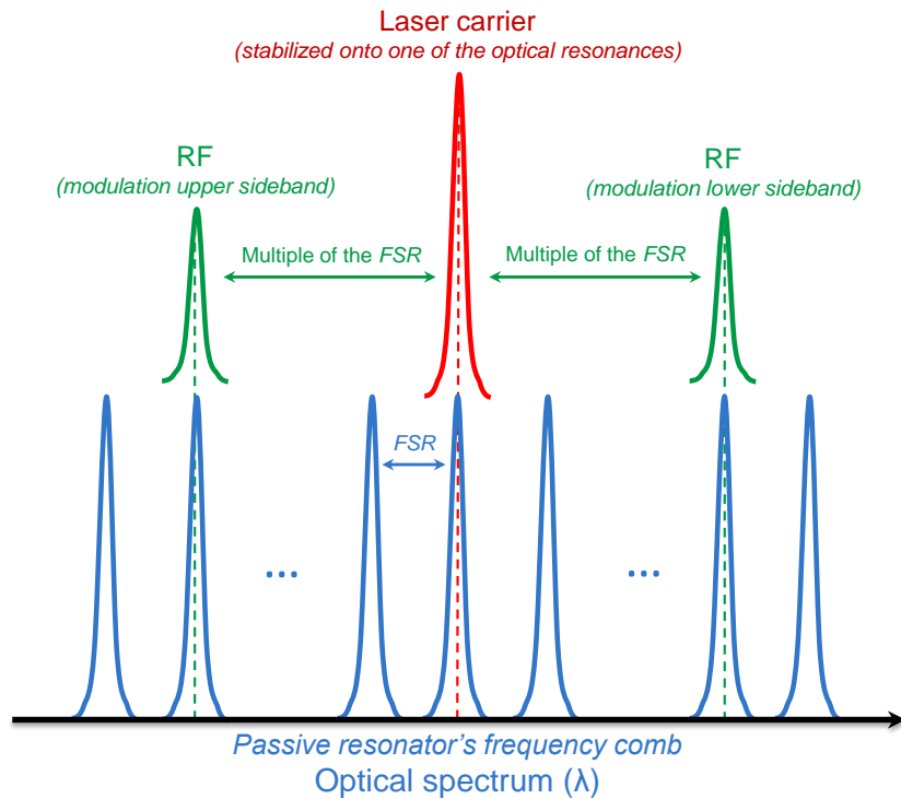
Fig. 1. Illustration of the microwave filtering using an optical frequency comb generated by an optical resonator.
