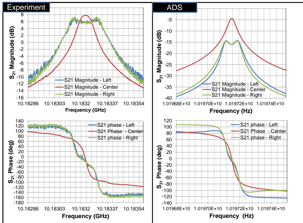
Fig. 8. Experimental and ADS simulation results of RF amplitude and phase responses of the OEO optical link in an open-loop configuration (laser + modulator + optical resonator + photodiode). Both results fit quantitatively well as they show that the resonance RF amplitude and phase responses are deformed when the laser frequency is stabilized onto one of the edges of the optical resonance.
