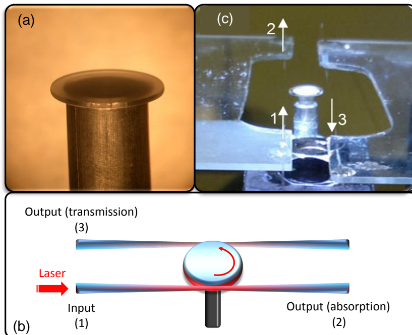
Fig. 3. (a) 5.5 mm-diameter whispering gallery mode \text{CaF}_2 disk-shaped micro-resonator fixed on a metallic rod; (b) illustration and (c) experimental setup of the symmetrical dual-coupling using two tapered optical fibers coupled to the \text{CaF}_2 disk.
