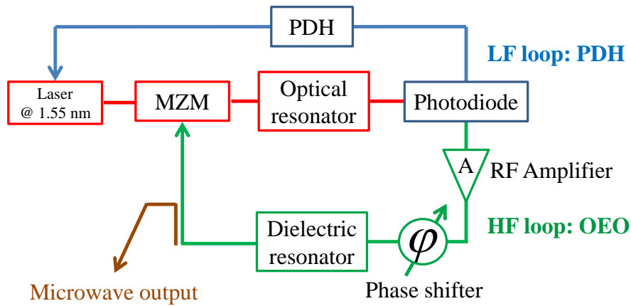
Fig. 2. OEO setup based on a low frequency (LF) PDH loop to stabilize the laser onto the resonator and a high frequency (HF) loop to maintain the microwave oscillation; PDH: Pound-Drever-Hall, MZM: Mach-Zehnder modulator.
