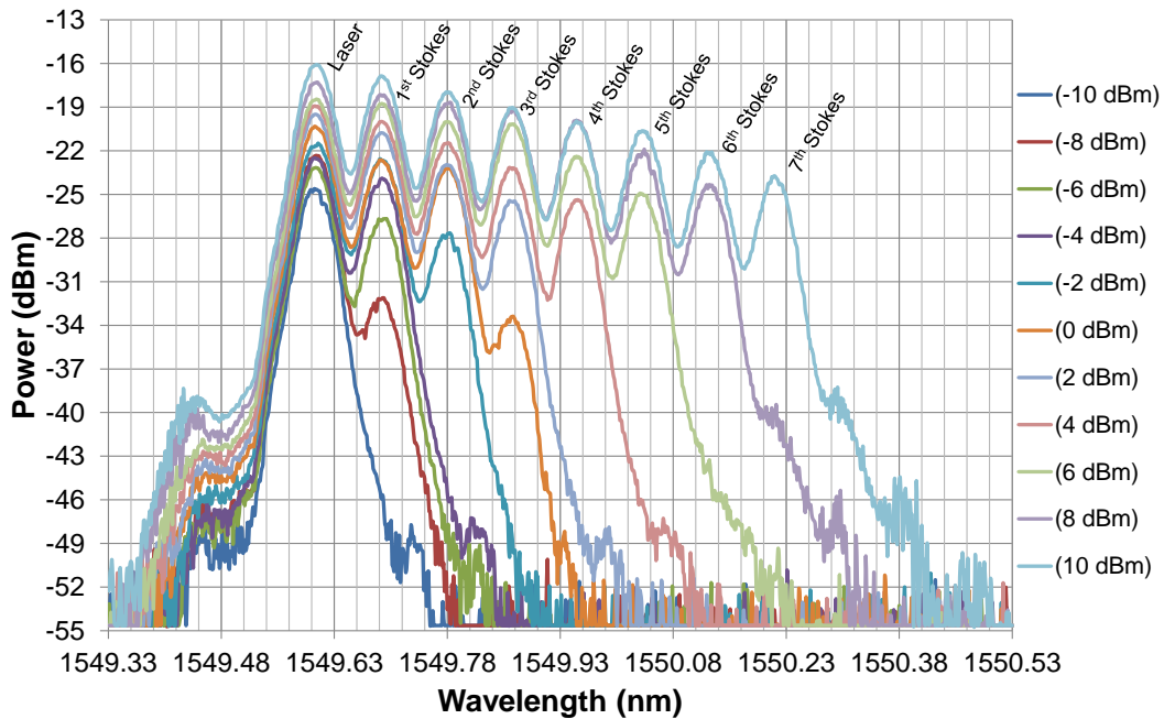
Fig. 9. Multiple stimulated Brillouin scattering lines generated inside a 20m-long fiber ring resonator featuring a Q_{Opt} factor of 3.5 \times 10^9 .
