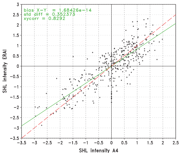
Figure 4. Scatter plot between the mean normalized intensity of the SHL derived from ERA-I (y-axis) and AMSU-A4 (x-axis) during established SHL phase (see text for more details). A linear regression has been added (green lines) and the characteristics of the distribution are indicated (top left), respectively the bias, the standard deviation and the temporal correlation.
