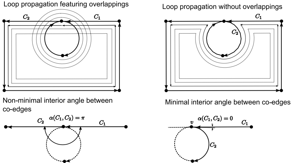
Fig. 12. Loops obtained regarding minimal interior angle criterion
