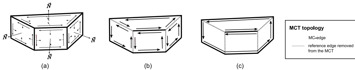
Fig. 11. Creation of co-edges : (a) co-edges oriented with the right-hand rule in the reference topology (b) orientation of reference edges underlying MC edges (c) orientation of MC edges inferred from the reference topology
