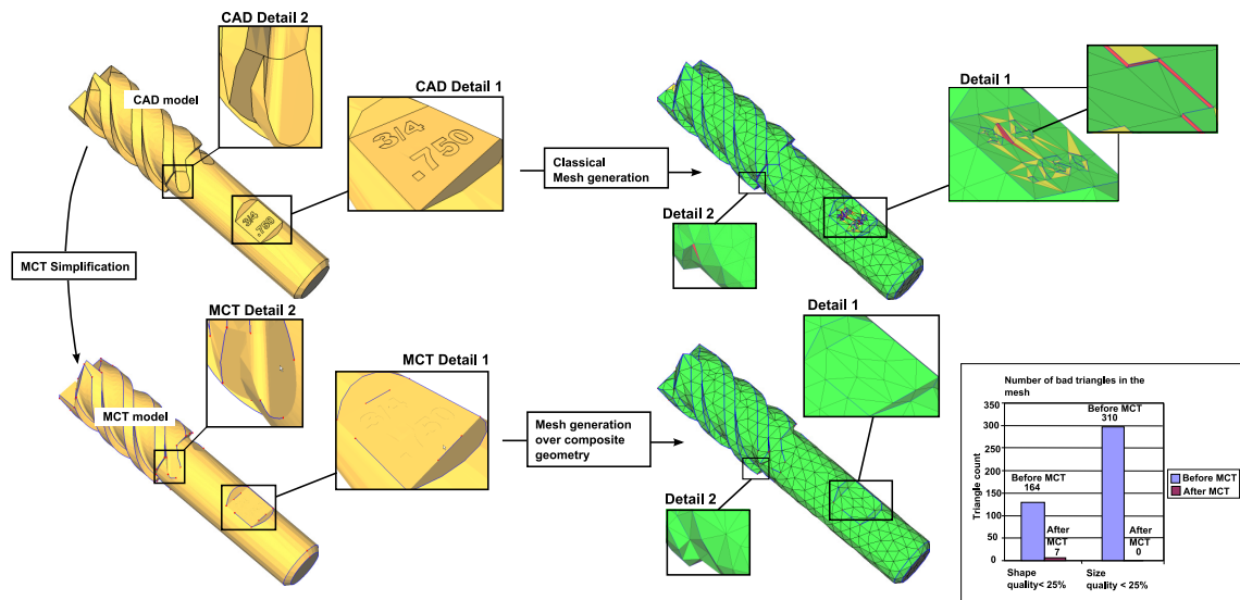
Fig. 30. Milling cutter: comparison between the meshes generated on the MCT model by composite surface meshing and on the initial (without preparation) CAD model.
