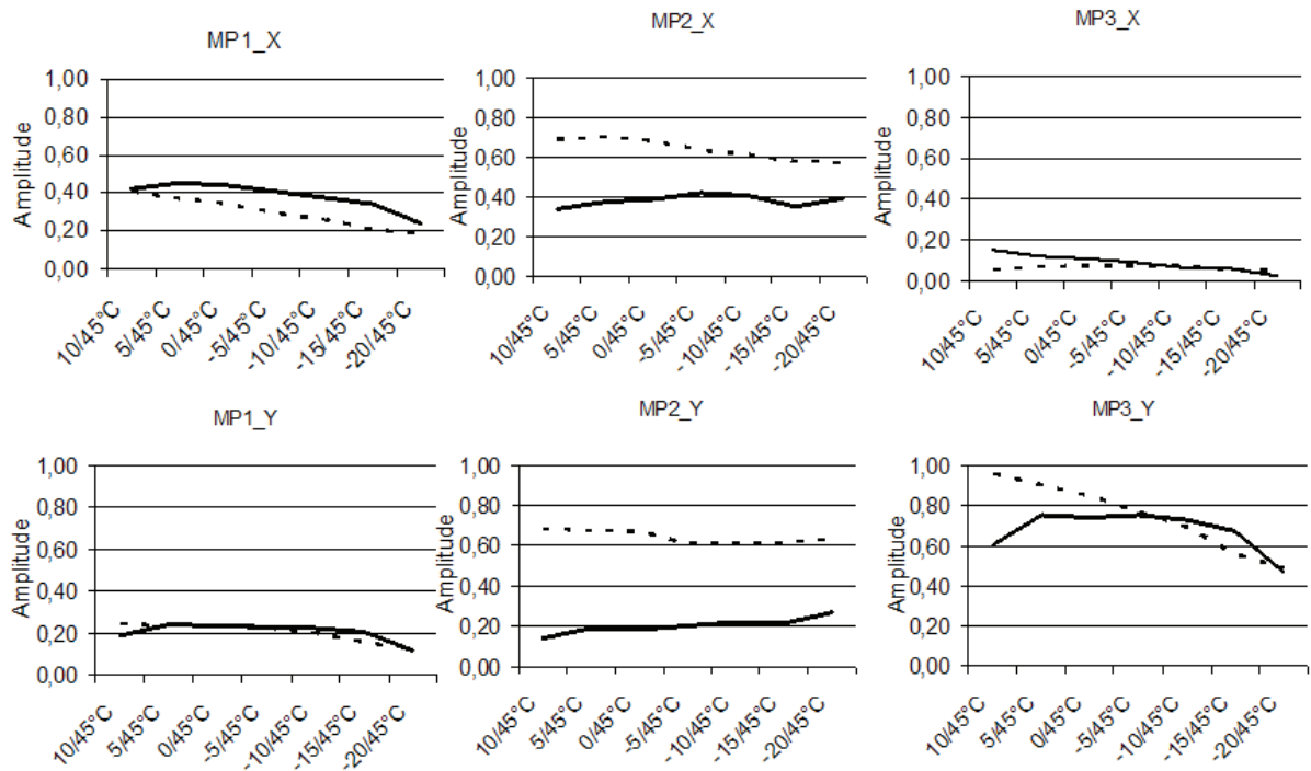
Figure 8. Dimensionless vibration levels versus operating conditions – X and Y directions at measurement points MP1, MP2 and MP3. Prototype#1 with proposed balancing (—), Prototype#2 with classical balancing (.....).
