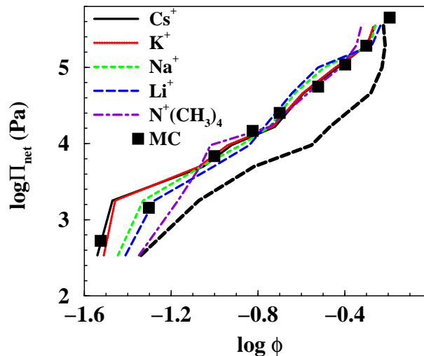
Figure 4: Osmotic pressures as a function of volume fraction for silica particles with a=10 nm and various counterions. Solid black line = \text{Cs}^+ , dotted red line = \text{K}^+ , short dashed green line = \text{Na}^+ and long dashed blue line = \text{Li}^+ . The dot-dashed violet line = \text{N}(\text{CH}_3)_4^+ and the dashed black line = \text{H}^+ , respectively. The simulated pressures are shown as filled squares. The bulk salt concentration is 0.5 mM.
