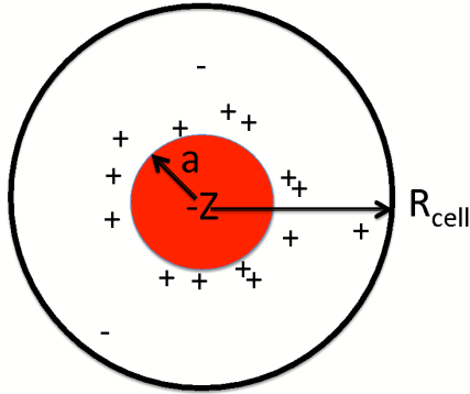
Figure 1: A central charged colloidal particle with radius a and a net charge Z is placed in a cell with radius R_{cell} . The cell is electroneutral and contains besides the counterions also salt pairs whose concentration is determined by an equilibrium with the surrounding bulk solution.
