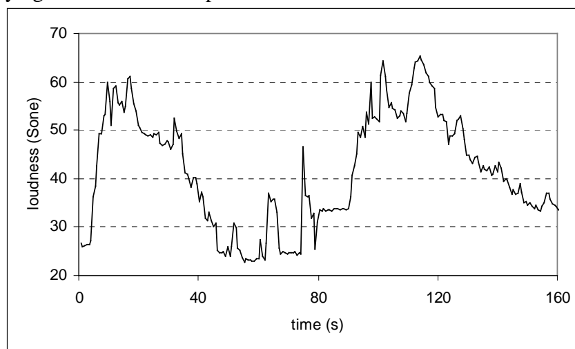
Figure 8: Loudness versus time of the signal.
