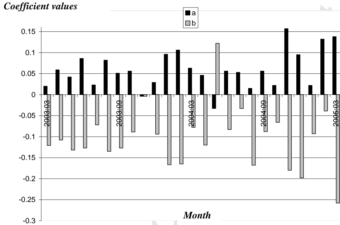
Figure 4: Month-by-month intercept and slope coefficients for regression of changes in relative confidence interval width on previous forecasting success
