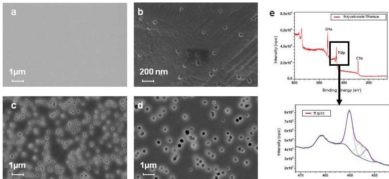
Fig. 1. Characterisation of plain and nanoporous titanium substrates by scanning electron microscopy and X-ray photoelectron spectroscopy. SEM micrographs of (a) Ti, (b) Ti30, (c) Ti150, (d) Ti300, and (e) representative XPS spectra of titanium-coated surfaces.
