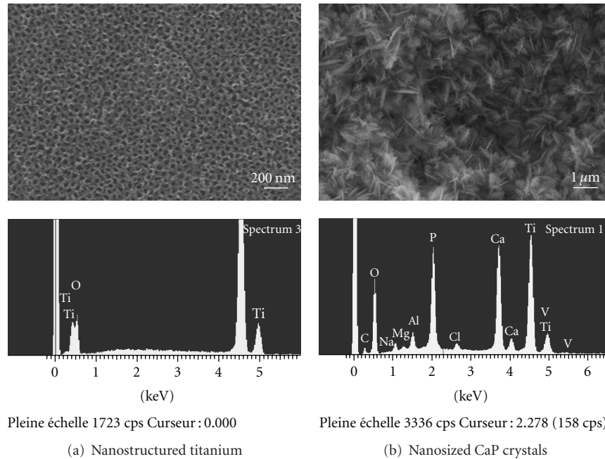
FIGURE 2: Scanning electron micrographs and energy dispersive analysis for X-ray of (a) nanostructured titanium surface obtained by anodization and (b) nanosized thin calcium phosphate (CaP) coating on titanium produced by electrochemical deposition. Note the regular array of TiO 2 nanopores of approximately 100 nm in diameter and the nanosized CaP crystals on titanium surfaces.
