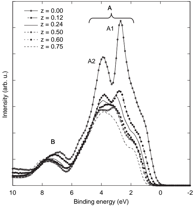
Fig. 5. Valence band photoemission spectra ( h\nu = 1486.6 eV) for z=0 up to 0.75. The binding energy is referred to the E_F at \text{BE}=0 eV. The A region is mainly based on Se 4p and Cu 3d interactions while B corresponds to the In–Se band.
