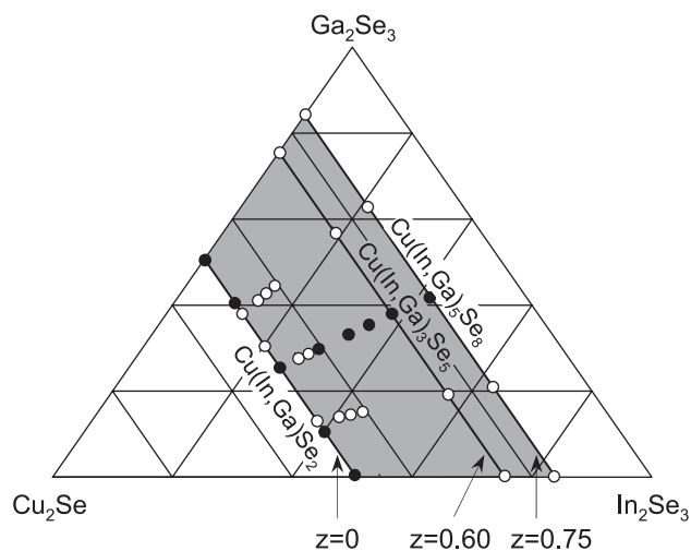
Fig. 1. Pseudo-ternary diagram in the \text{Cu}_2\text{Se} – \text{In}_2\text{Se}_3 – \text{Ga}_2\text{Se}_3 system showing the composition of all synthesized compounds. Only the compounds corresponding to black circles are presented in this study.
