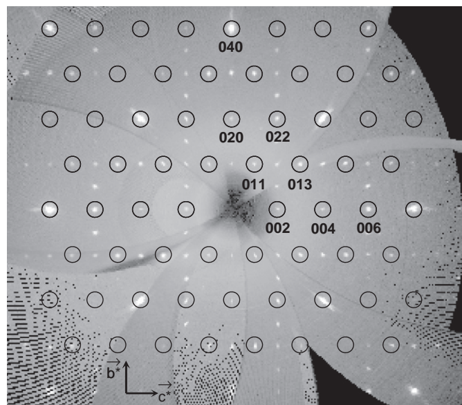
Fig. 3. Precession image of 0kl plane for the \text{Cu}_{0.5}(\text{In}_{0.5}\text{Ga}_{0.5})_{1.17}\text{Se}_2 compound. The indexed reflections (circles) correspond to the tetragonal unit cell ( a=5.6450 \text{ \AA} and c=11.2438 \text{ \AA} ) and the others are due to twinning along the [2\ 2\ 1] direction.
