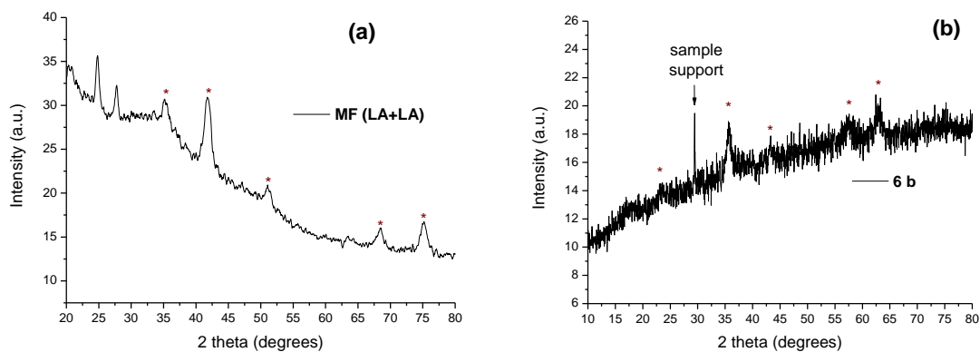
Figure 2. XRD spectra for: (a) MF (LA+LA); (b) magnetic nanoparticles 6b .
