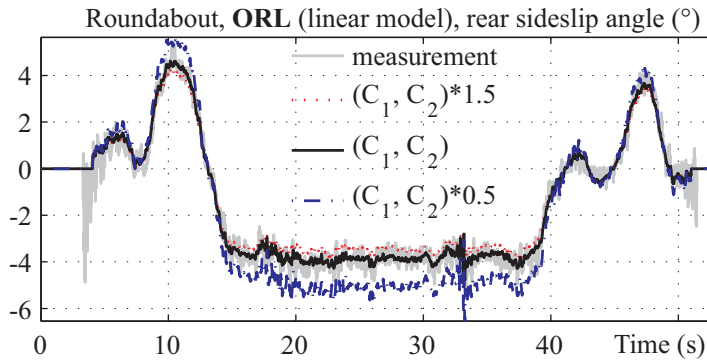
Fig. 13. ORL observer (linear tire-force model) , rear sideslip angle estimates, with different stiffness settings.
