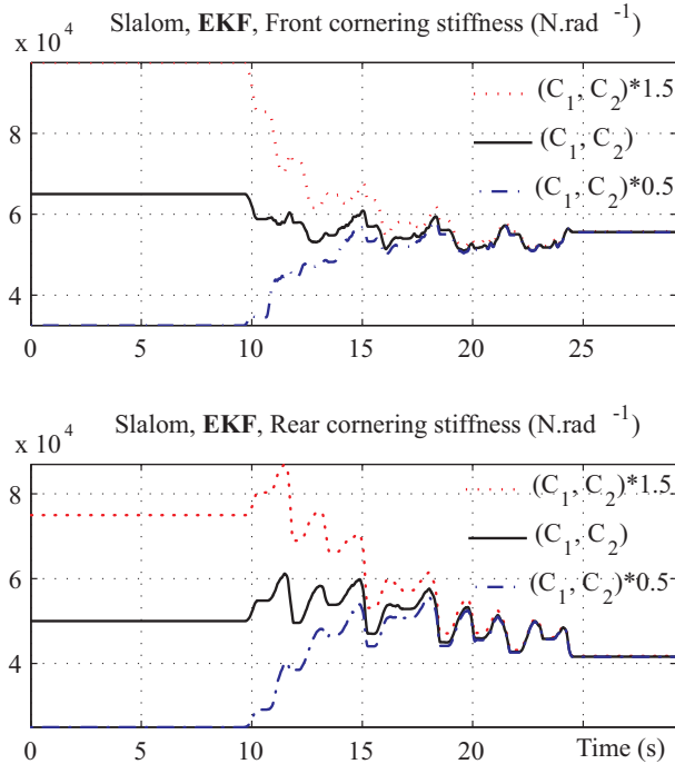
Fig. 16. Slalom test, EKF observer (linear adaptive force model) , with different cornering stiffness settings [(C_1, C_2) = (65000, 50000) * (0.5, 1, 1.5) N.rad^{-1}] . Front and rear cornering stiffness estimates C_i + \Delta C_{ai} .
