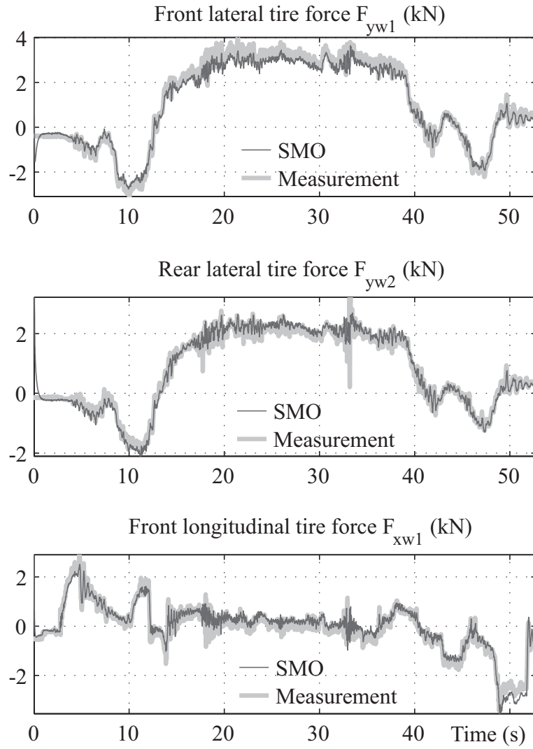
Fig. 8. Roundabout. SMO observer. Tire force estimates.
