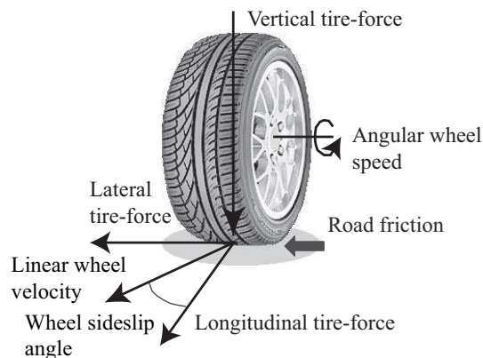
Fig. 1. Wheel dynamic variables.
