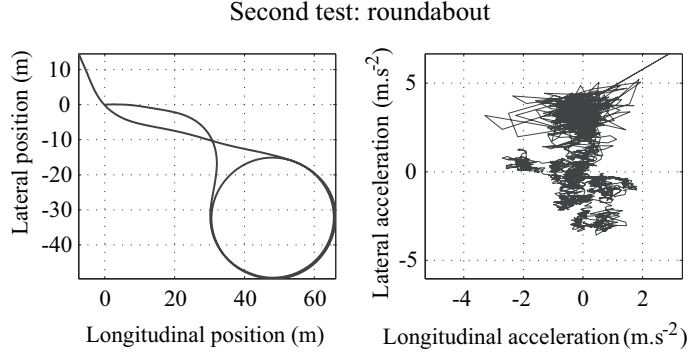
Fig. 6. Roundabout experimental test, vehicle position, acceleration diagram.
