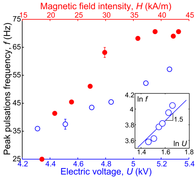
Figure 5. Experimental dependences of peak pulsations frequency on electric voltage (○, at H = 27 kA/m, d = 630 \mu m) and on external magnetic field intensity (●, at U = 4.1 kV, d = 775 \mu m).
