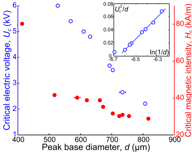
Figure 3. Experimental dependences of critical electric voltage ( \circ , at H = 27 kA/m) and critical magnetic field intensity ( \bullet , at U = 3 kV) at which electrocapillary instability occurs on peak base diameter.
