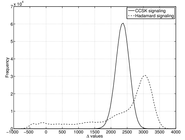
Fig. 6. Histograms of \Delta for CCSK and Hadamard signaling over a constant 2-path channel in phase opposition ( \frac{E_b}{N_0} \approx 15 dB)
