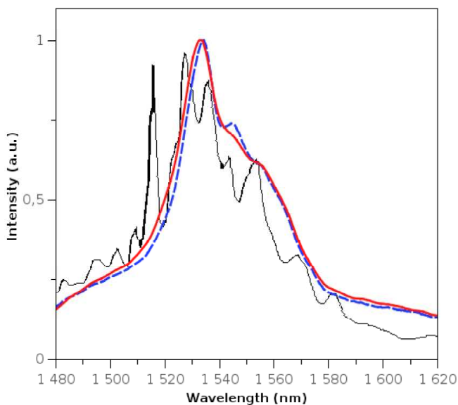
Figure 3. Room temperature emission under 980-nm excitation. Blue dashed line: [Mg] sol = 0.5 mol/l and no phosphorus. Red solid line: [Mg] sol = 1.0 mol/l with phosphorus. FWHM = 39.5 and 42.7 nm, respectively. Resolution: 2 nm. Thin black line: attributed to Er-doped MgSiO 3 units, from [11]
