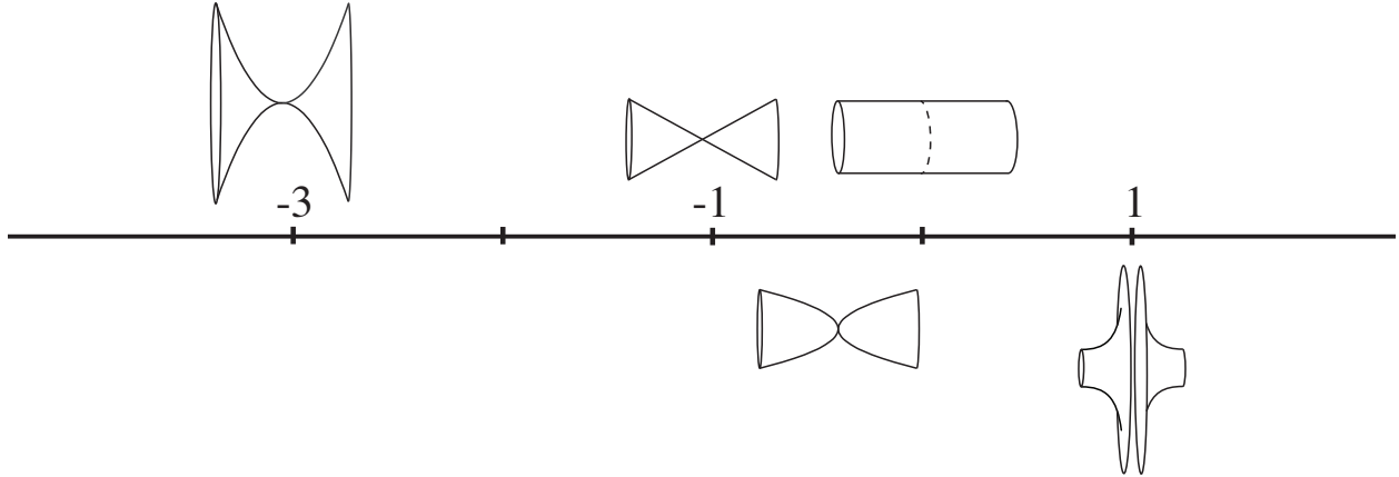
FIGURE 1. Geometric interpretation of M_\alpha . The figures above the line are isometric to M_\alpha , while for the ones below the isometry is singular in a neighborhood of \mathcal{Z} .
