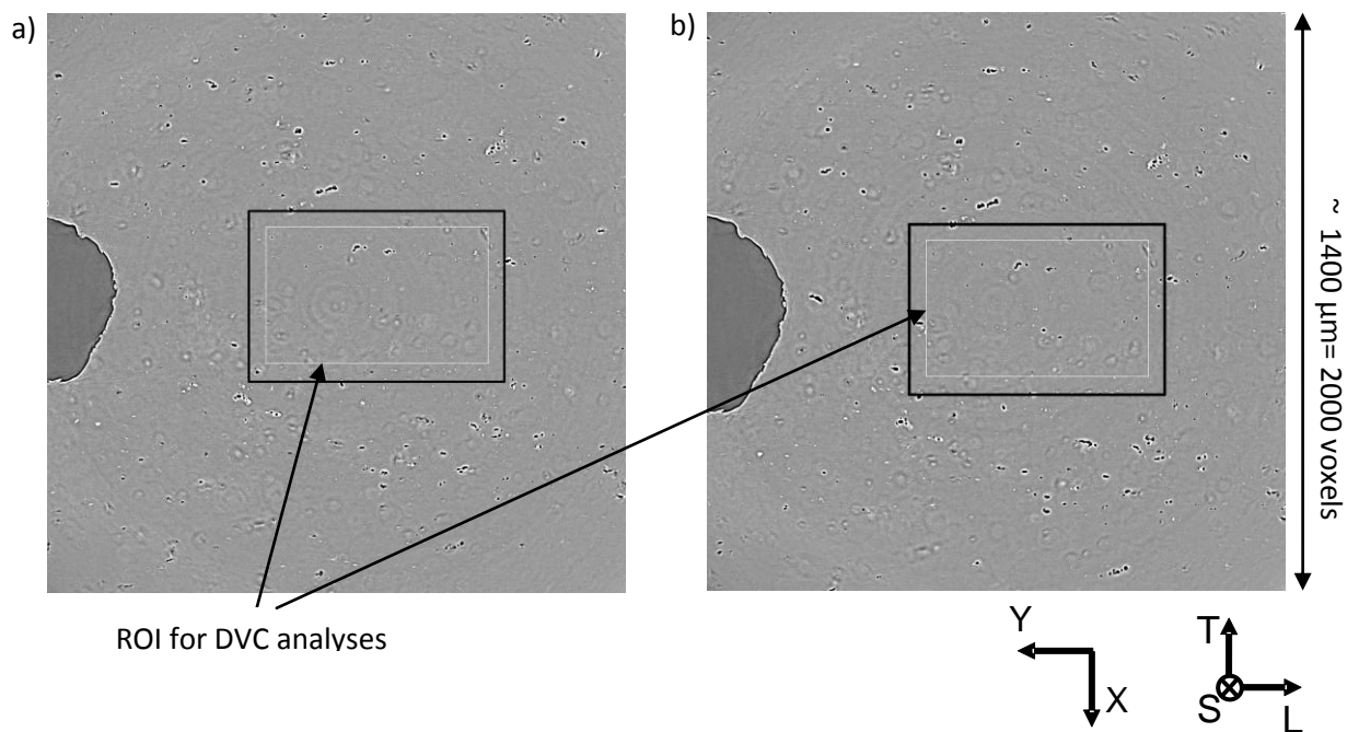
Figure 12: 2D sections of reconstructed laminography data at mid thickness showing the location of the extracted volume (600 x 900 x 300 voxels) in black and the ROIs
