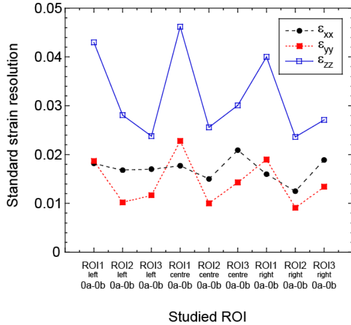
Figure 7: Standard strain resolutions along the three directions as functions of the studied ROI for the rigid-body-motion/resolution analysis ( \ell = 16 voxels).
