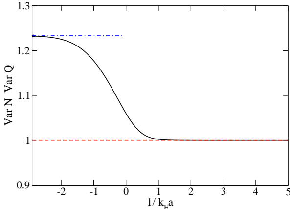
FIG. 4: (Color online) Product of the variances of the phases with the variance of the number of particles at time t = 0 for a system in the BCS ground state. The black solid line shows \text{Var} \hat{Q}(0) \text{Var} \hat{N} , the dashed red line \text{Var} \hat{\theta}_0(0) \text{Var} \hat{N} , and the blue dashed dotted line is the BCS limit of \text{Var} \hat{Q}(0) \text{Var} \hat{N} . The expression of \text{Var} \hat{Q}(0) is given by (B5) and the one of \text{Var} \hat{N} by equation (93).
