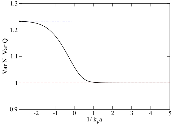
FIG. 4: (Color online) Product of the variances of the phases with the variance of the number of particles at time t = 0 for a system in the BCS ground state. The black solid line shows \text{Var} \hat{Q}(0) \text{Var} \hat{N} , the dashed red line \text{Var} \hat{\theta}_0(0) \text{Var} \hat{N} , and the blue dashed dotted line is the BCS limit of \text{Var} \hat{Q}(0) \text{Var} \hat{N} . The expression of \text{Var} \hat{Q}(0) is given by (B5) and the one of \text{Var} \hat{N} by equation (93).
