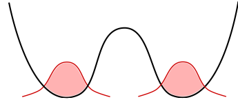
FIG. 6: The gas is split into two components by adiabatically changing the single-well potential of Fig. 5 to a double-well potential
