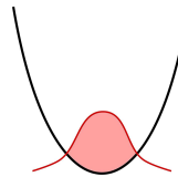
FIG. 5: Ideal gas of bosonic dimers initially in a single-well trap
