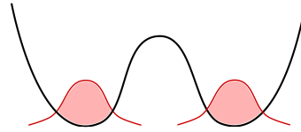
FIG. 6: The gas is split into two components by adiabatically changing the single-well potential of Fig. 5 to a double-well potential
