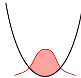
FIG. 5: Ideal gas of bosonic dimers initially in a single-well trap
