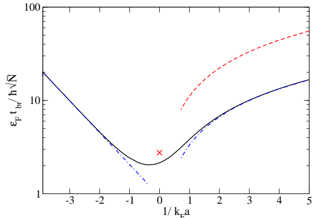
FIG. 3: (Color online) Phase blurring time t_{\text{br}} in the BCS ground state (solid line). The dashed-dotted blue lines show the asymptotic behaviors. The dashed red line is the exact asymptotic behavior and the red cross is the expected value for k_F|a| = \infty . In all cases we take \text{Var } \hat{N} as given by the BCS ground state.
