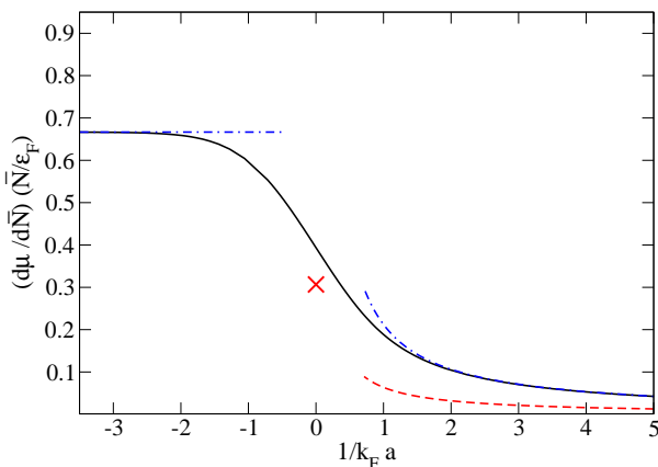
FIG. 2: (Color online) d\mu/d\bar{N} in the BCS ground state. The full line is the BCS mean field approximation, the dashed-dotted blue lines show the asymptotic behaviors. The dashed red line is the exact (beyond BCS theory) asymptotic behavior on the BEC side and the red cross is the value at the unitary limit k_F|a| = \infty deduced from the value of the universal parameter \xi in the equation of state [23].
