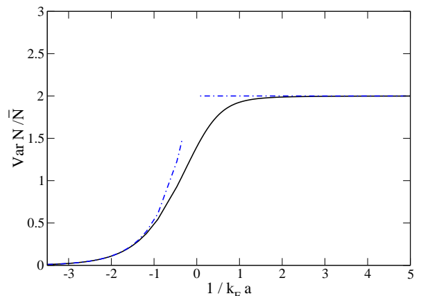
FIG. 1: (Color online) Variance of the total particle number \hat{N} in the BCS ground state (solid line). The dashed-dotted blue lines are the asymptotic behaviors in the BEC or BCS limits.
