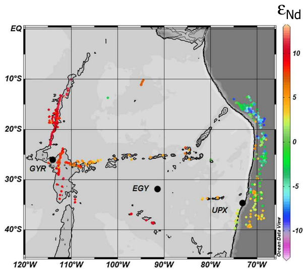
Figure 6. Map of the distribution of \epsilon_{Nd} in the outcropping rocks and sediments at the surface of the continent and at the sea bottom. The radiogenic values close to station GYR are distributed along the East Pacific Rise, and the Easter-Salas y Gomez Seamount Chain in the east. Topographic lines are marking the depths of 3000 m, 2500 and 2000 m.
