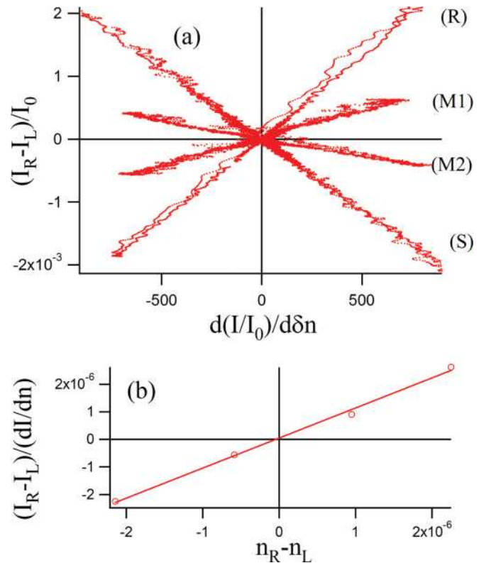
FIG. 3. (Color online) (a) Experimental difference of transmission between left and right circular waves as a function of the derivative of the total transmitted light with respect to the difference of refractive indices \delta n . Solutions are oil with limonene ( R ) and ( S ) and mixes ( M1 ) and ( M2 ) of ( R ) and ( S ). (b) Measured slopes from (a) plotted as a function of \Delta n ; the solid line corresponds to Eq. (8).
