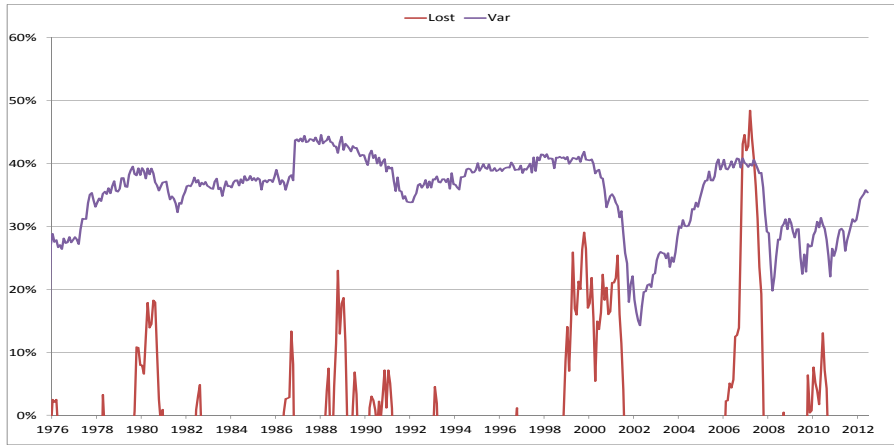
Figure 17: MSCI 1 year VaR
