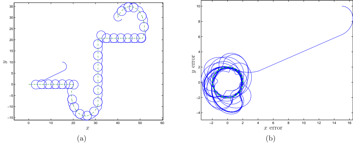
Figure 19: Time-optimal based tracking method in 2D. UAV's trajectory is continuous, target's trajectory is dashed and the \mathcal{C}_t is dashed. The behavior of the target is known. (x_0, y_0, \theta_0) = (15, 10, 0) , (z_1, z_2) = (0, 0) , and u_{\max} = -a = 0.5 . (a) Trajectories drawn in the (x, y) -coordinates plane. (b) Trajectories drawn in a (orthonormal) frame attached to the center of \mathcal{C}_t .
