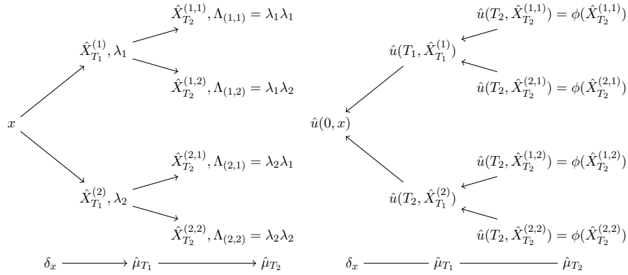
FIGURE 1. Left: Cubature tree. Right: Backward scheme.
