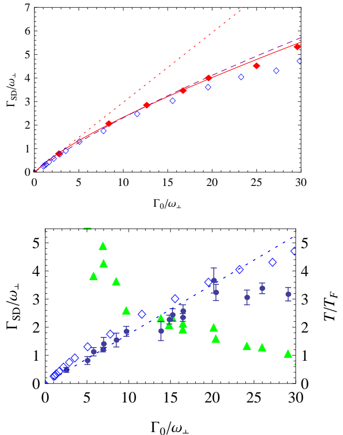
FIG. 3: (Color online). Spin-drag coefficient \Gamma_{SD} in a harmonic trap. Top: theoretical predictions. For a constant cross-section the red solid diamonds are the results of the molecular dynamics simulation and the red solid line is the numerical resolution of the eigenequation (3). For a momentum dependent cross-section close to the unitary limit ( k_{th}a = 2 , with k_{th} = \sqrt{k_B T/\hbar^2} the thermal wave-vector), the blue open diamonds correspond to the molecular dynamics simulation while the blue dashed line is the solution of Eq. (3). The red dotted line is the collisionless prediction \Gamma_{SD} = \Gamma_0/4.03 for a unitary gas. Bottom: comparison with the experimental results of Ref. [15] at unitarity (blue dots). The green triangles represent the associated values of T/T_F . As above, the blue open diamonds correspond to the molecular dynamic simulation at k_{th}a = 2 . Blue-dotted line: experimental fit \Gamma_{SD} \simeq \Gamma_0/5.7 . For the experimental data, \Gamma_0 is calculated using the theoretical value Eq. (4) for the unitary gas.
