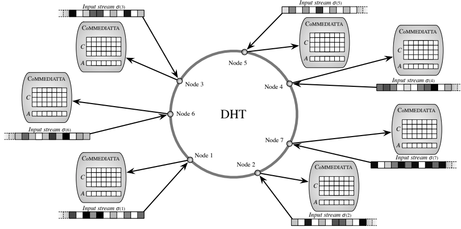
Fig. 1: CoMEDIA structure, where each node runs a CoMMEDIETTA instance over a DHT.
