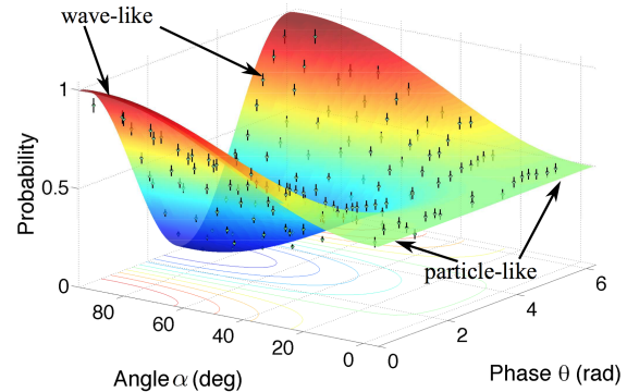
FIG. 2. Continuous morphing from wave to particle-like behaviours when manipulating the QBS at the output of our MZI (see FIG. 1). \theta is a tunable phase in one arm of the interferometer, while \alpha is the polarization state analysis angle of the corroborative photon.
