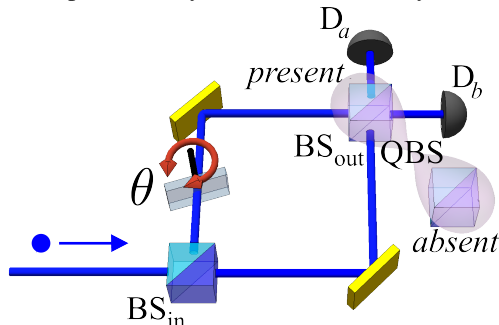
FIG. 1. Setup for observing single photon wave-particle complementarity based on a MZI. When the output beam-splitter ( BS_{out} ) is absent, a click on detector D_a or D_b reveals a particle behaviour. When BS_{out} is present, phase ( \theta ) dependent intensity oscillations are observed in these detectors, revealing a wave phenomenon [3, 4]. In our quantum version of Wheeler's experiment, BS_{out} is prepared in a coherent superposition of being present and absent by exploiting entanglement, leading to the implementation of a quantum beam-splitter (QBS) [5, 6].
