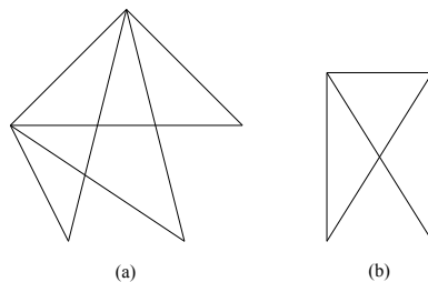
FIGURE 1. (a) K_{[5,3]} and (b) K_{[4,2]}
